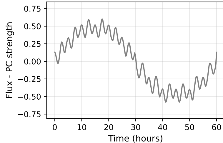
A — i=20^\circ Light Curve
