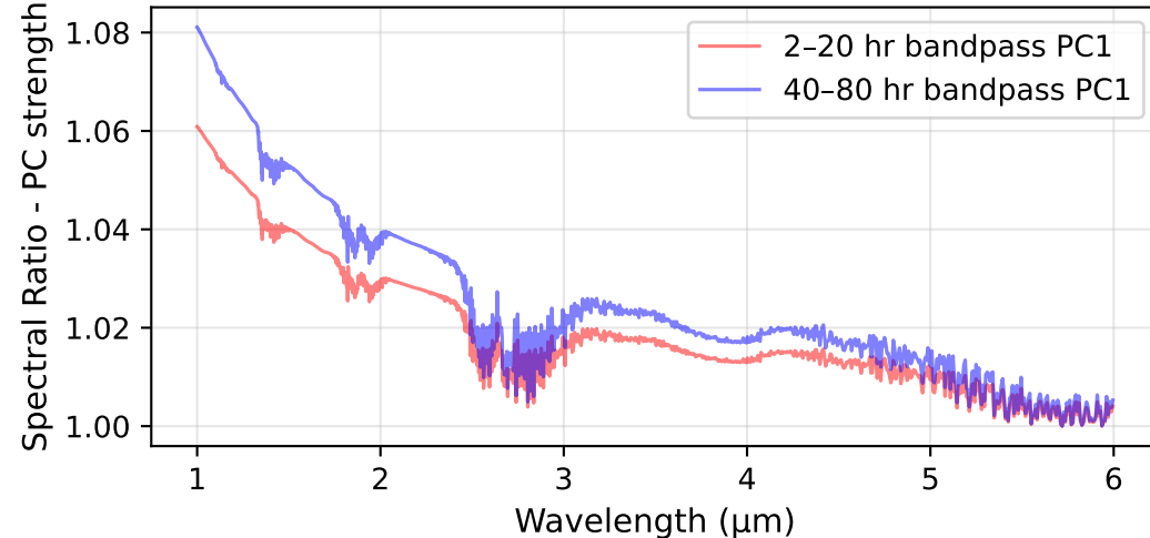
C — i=20^\circ Bandpass filtered Spectral Ratio
