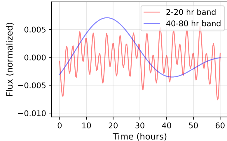
B — i=20^\circ Bandpass filtered light curves
