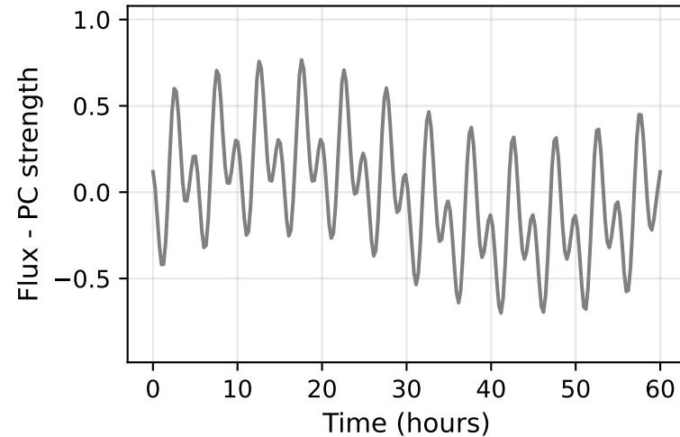
A — i=40^\circ Light Curve
