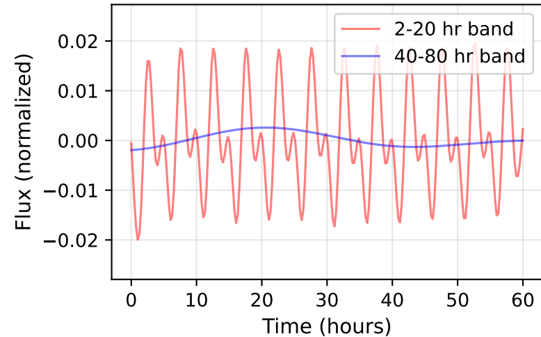
B — i=40^\circ Bandpass filtered light curves
