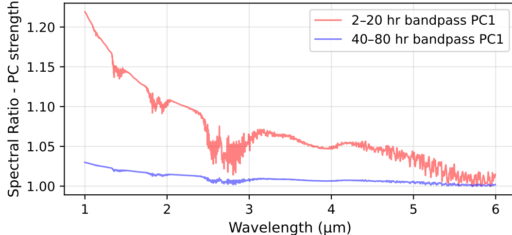
C — i=40^\circ Bandpass filtered Spectral Ratio
