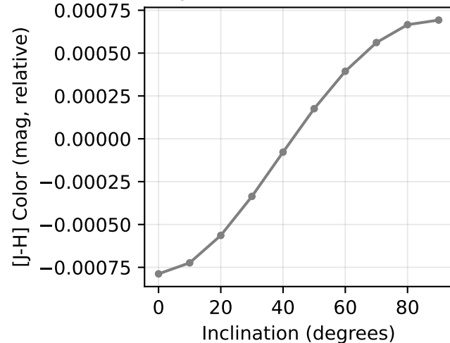
[J-H] Color vs Inclination
