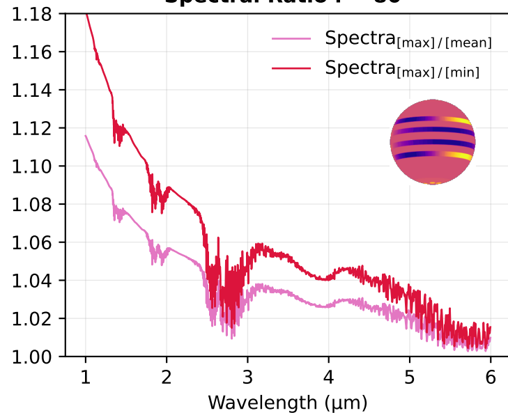
Spectral Ratio i = 80^\circ
