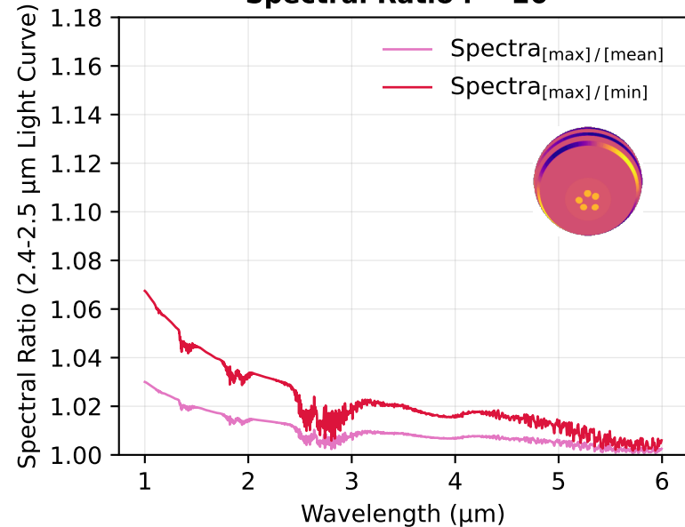
Spectral Ratio i = 20^\circ
