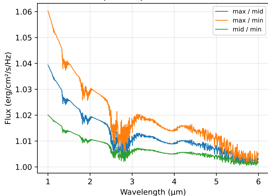
Composite Spectra Ratio; i=20
