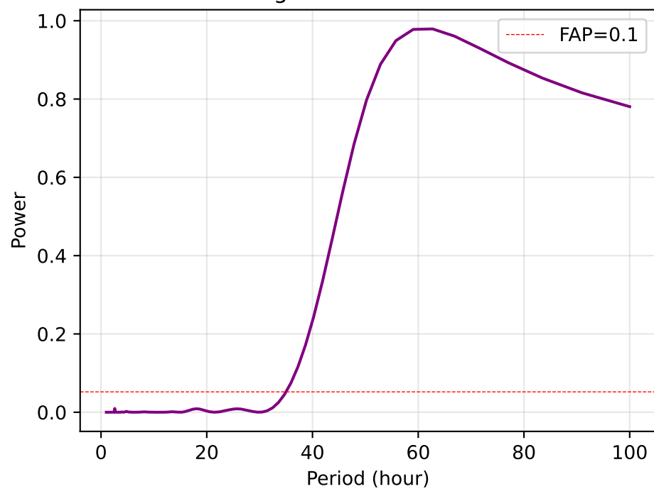
Periodogram of Flux Timeseries
