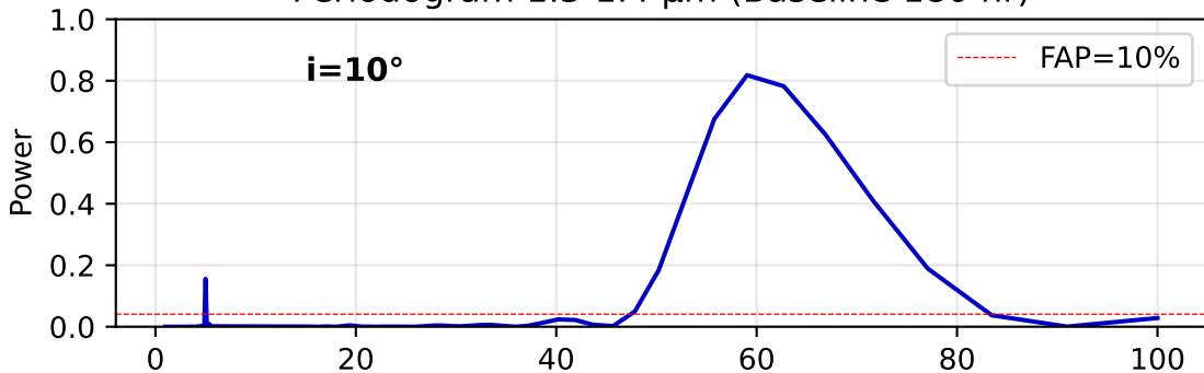
Periodogram 1.3-1.4 \mu\text{m} (Baseline 180 hr)
