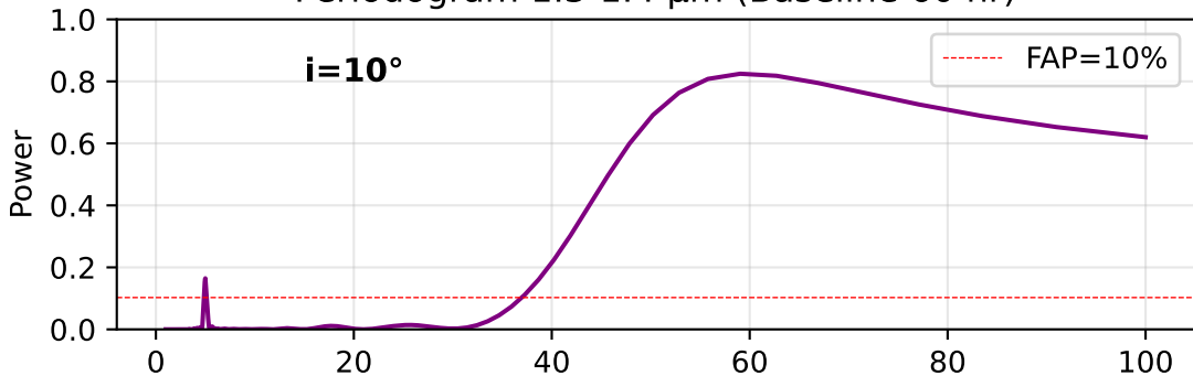
Periodogram 1.3-1.4 \mu\text{m} (Baseline 60 hr)
