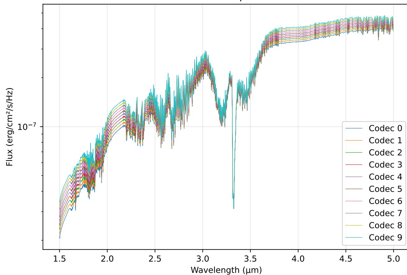
Fractional Contributions (Frame 0); i=40
