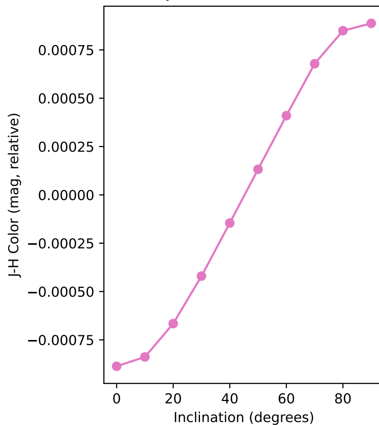
J-H Color vs Inclination
