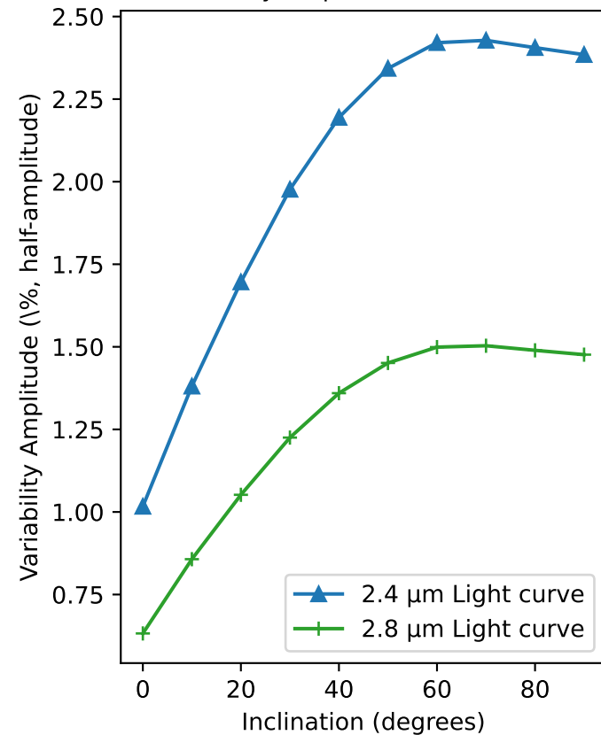
Variability Amplitude vs Inclination
