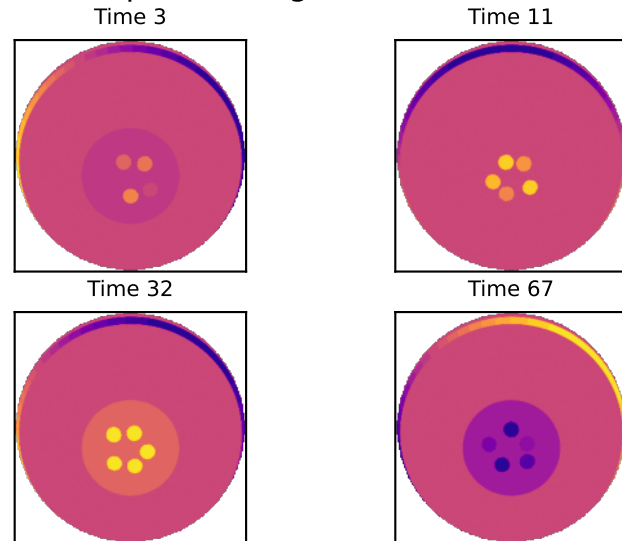
Atmosphere Images at Selected Times
