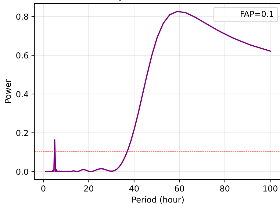
Periodogram of Flux Timeseries
