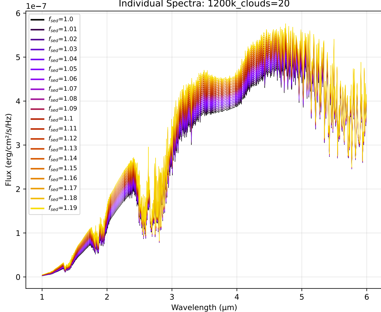
Individual Spectra: 1200k_clouds=20
