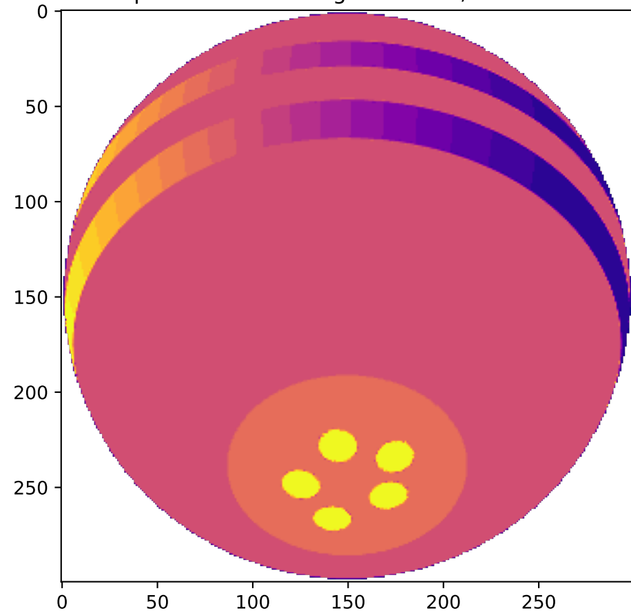
Spectral-codec Image at i=40^\circ , frame 23
