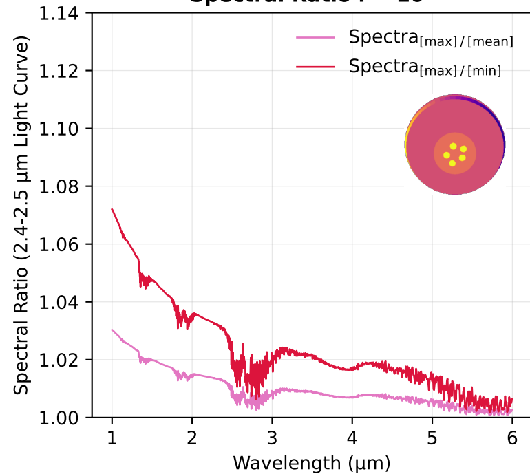
Spectral Ratio i = 10^\circ
