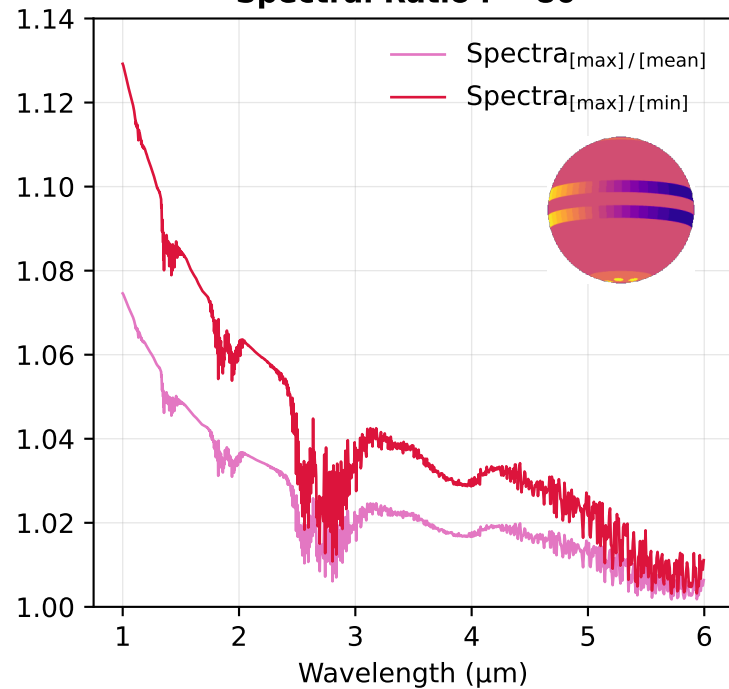
Spectral Ratio i = 80^\circ
