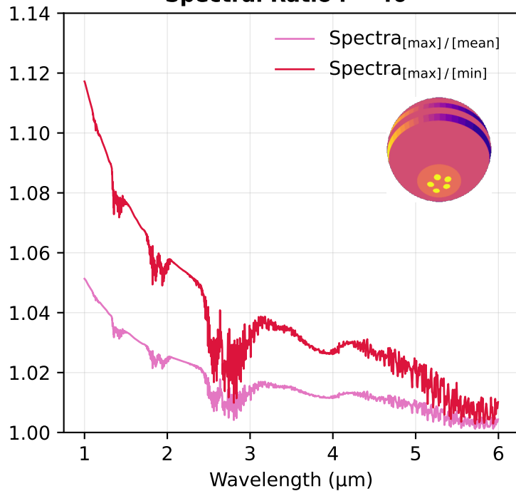
Spectral Ratio i = 40^\circ
