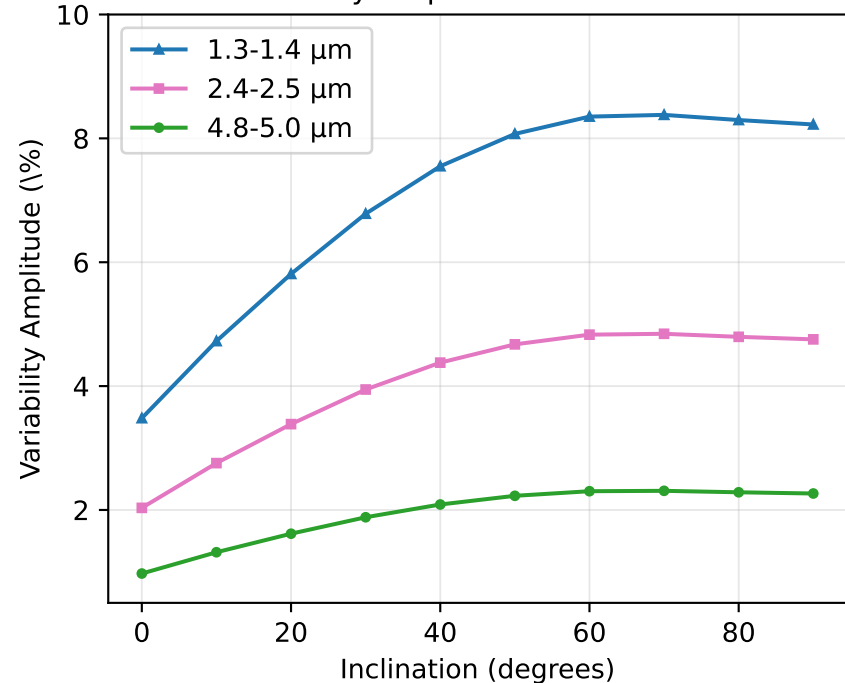
Variability Amplitude vs Inclination
