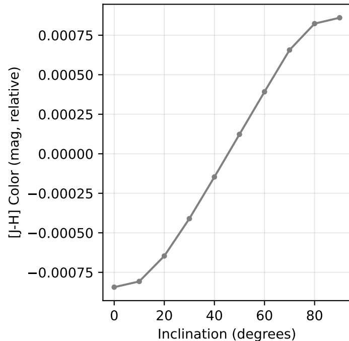
[J-H] Color vs Inclination
