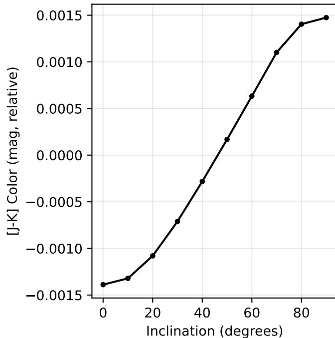
[J-K] Color vs Inclination
