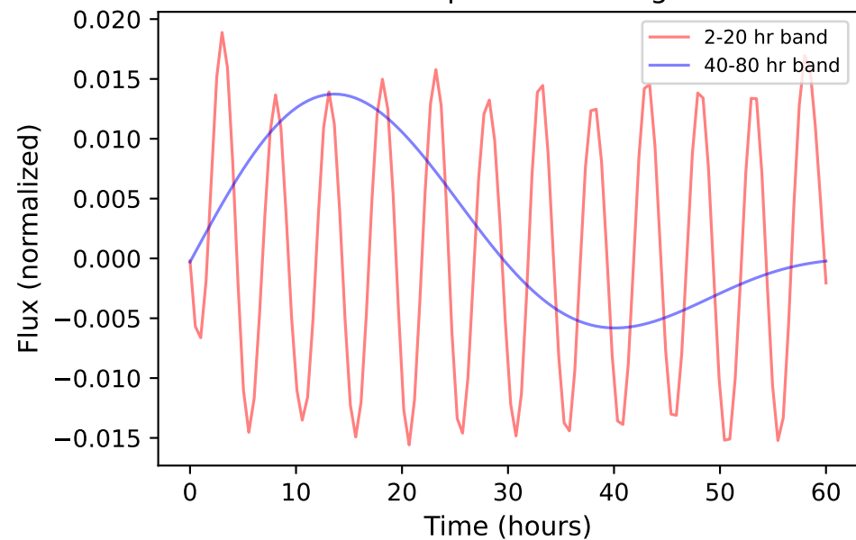
C — i=20^\circ Bandpass filtered light curves
