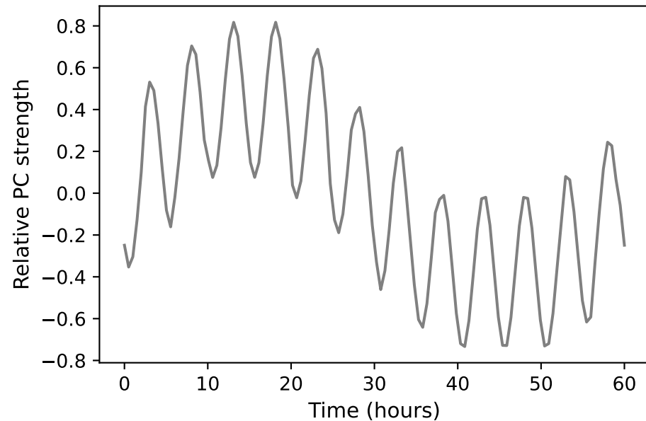
D — PCs of bandpass filtered spectra for i=20^\circ
