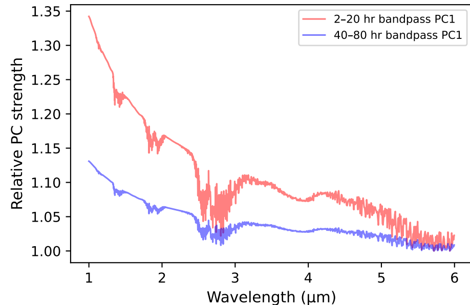
D — PCs of bandpass filtered spectra
