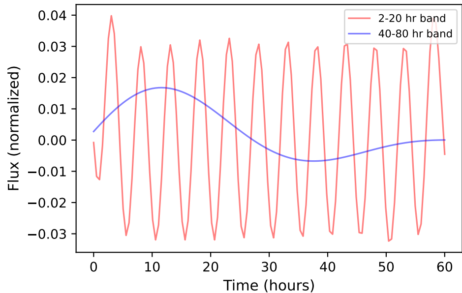
C — i=50^\circ Bandpass filtered light curves
