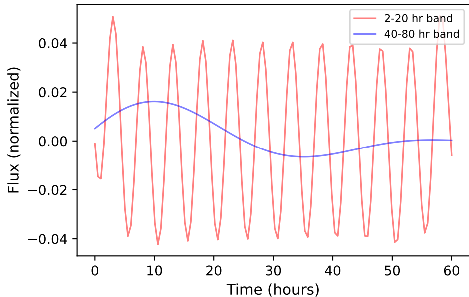
C — i=90^\circ Bandpass filtered light curves
