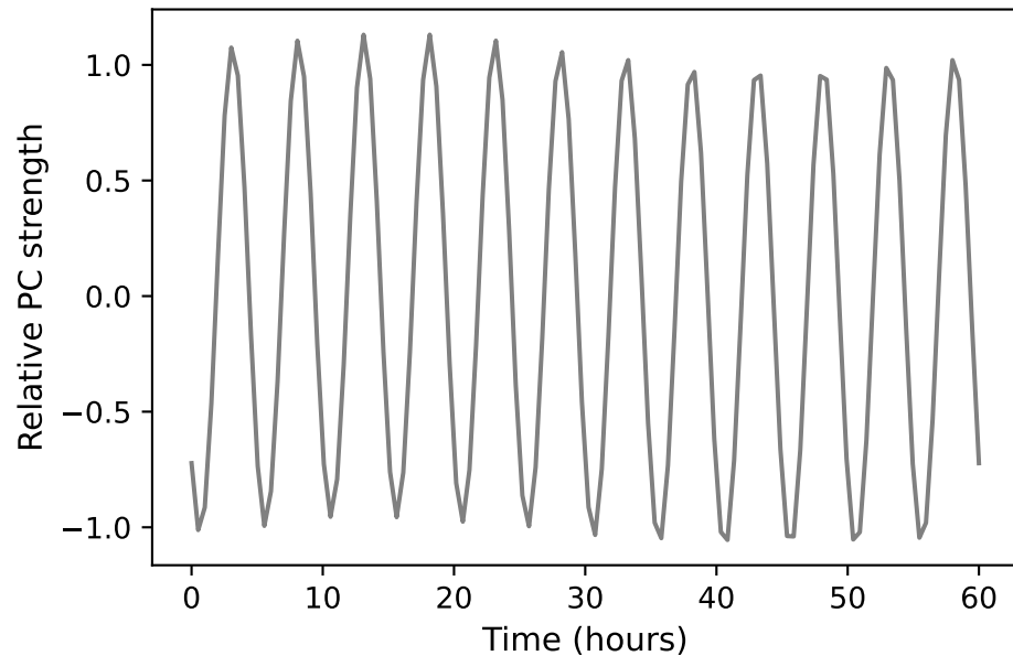
D — PCs of bandpass filtered spectra for i=90^\circ
