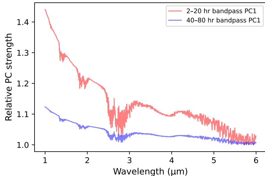
D — PCs of bandpass filtered spectra for i=90^\circ
