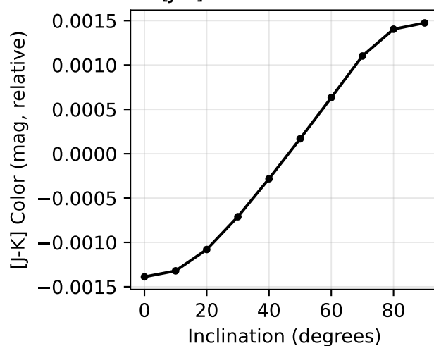
[J-K] Color vs Inclination
