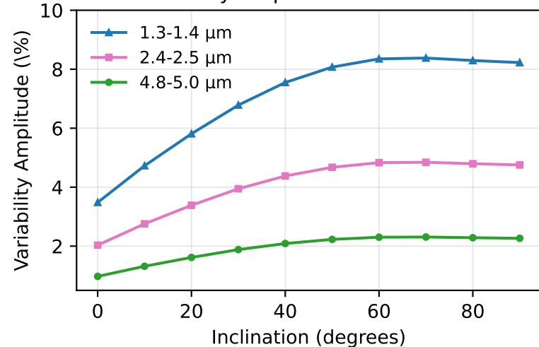
Variability Amplitude vs Inclination
