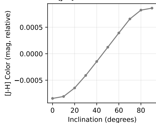
[J-H] Color vs Inclination
