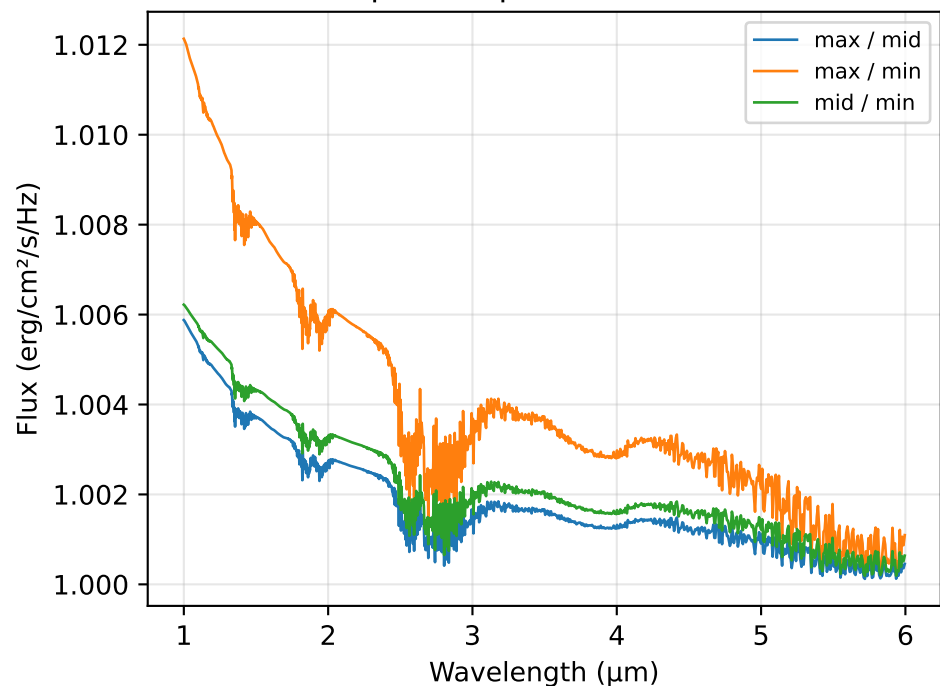
Composite Spectra Ratio; i=30
