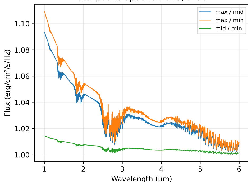
Composite Spectra Ratio; i=50
