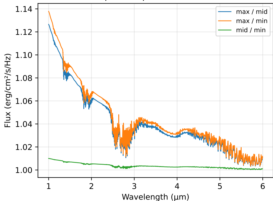
Composite Spectra Ratio; i=60
