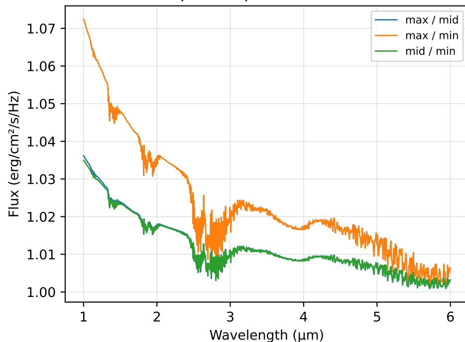
Composite Spectra Ratio; i=30
