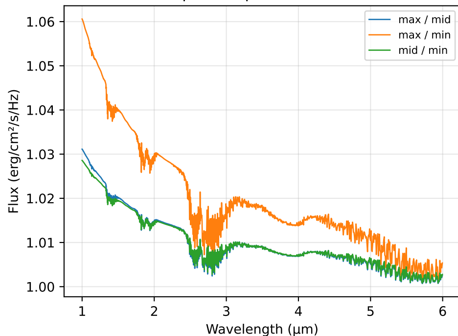
Composite Spectra Ratio; i=0
