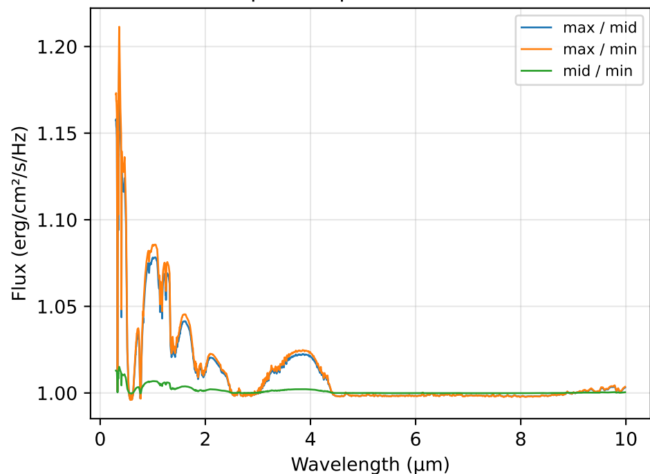
Composite Spectra Ratio; i=60
