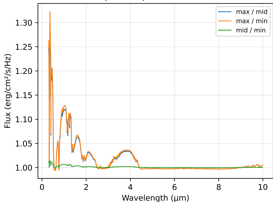
Composite Spectra Ratio; i=90
