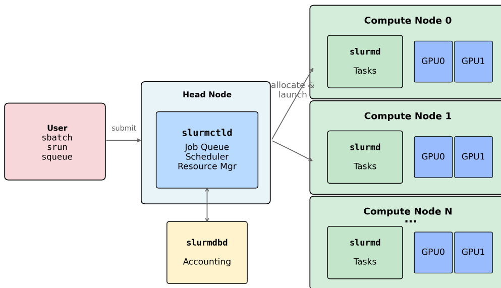
Figure 8.1: SLURM Architecture: slurmctld , slurmmd , and slurmdbd daemons.
