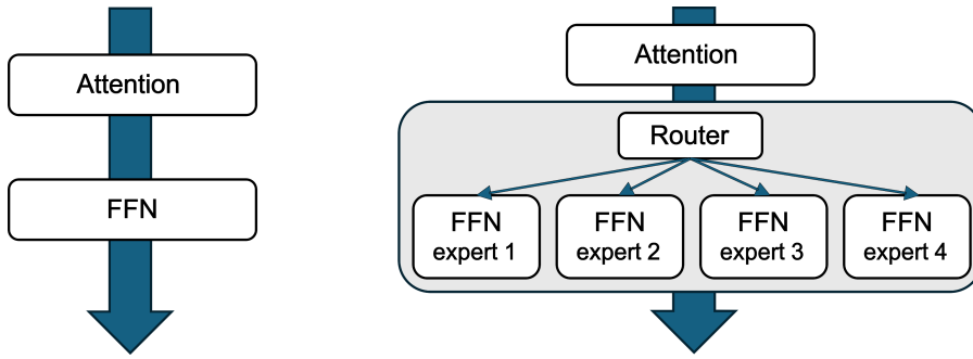
Figure 6.13: MoE architecture
