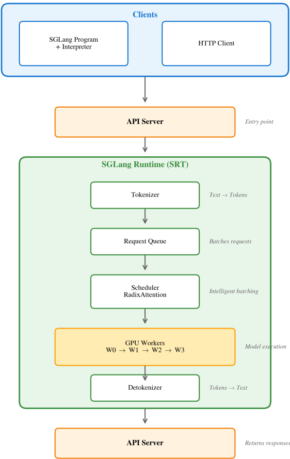
Figure 7.1: SGLang Architecture
