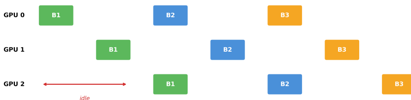
Figure 6.12: Pipeline bubble
