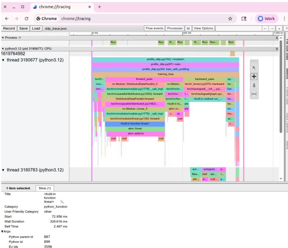
Figure 3.10: Chrome Tracing View of a DDP Run
