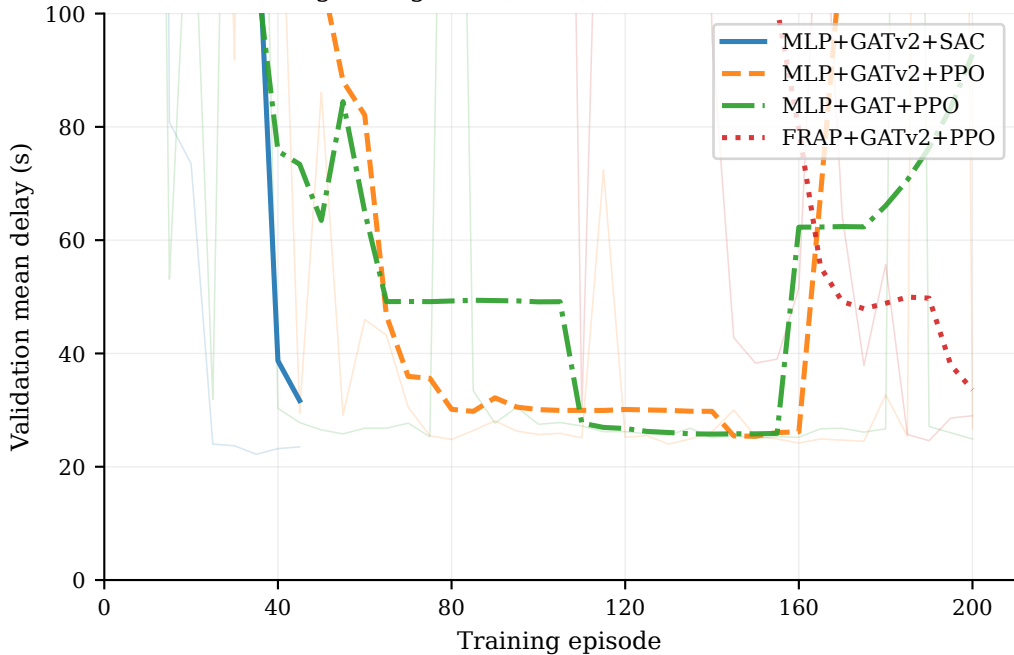
Cologne Regional ( N = 8 ) — ablation variants
