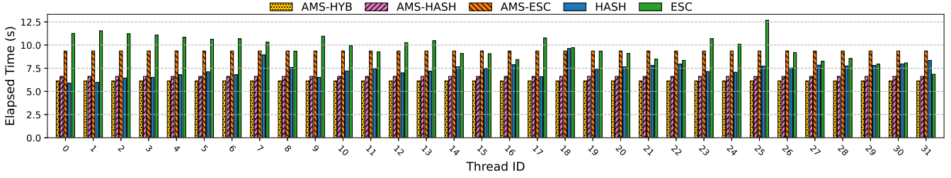
Figure 11: Per-thread elapsed time of the numeric phase comparison of AMS-based variants (AMS-HYB, AMS-HASH, AMS-ESC) and their baseline counterparts (HASH, ESC) on a G500 skewed matrix (scale=19, edgefactor =8).
