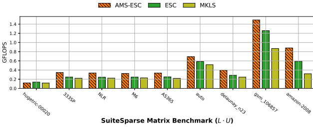
Figure 22: Triangle counting throughput on nine SuiteSparse matrices.
