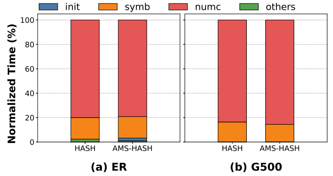
Figure 25: Normalized end-to-end runtime breakdown on ER and G500 at scale 19, edgefactor 16, where every bar is normalized to its own end-to-end SpGEMM time. Each bar is partitioned into the symbolic phase ( symb ), the numeric phase ( numc ), AMS’s morsel preparation ( init ), and the remaining management steps of prefix sum, output allocation, and finalization ( others ).
