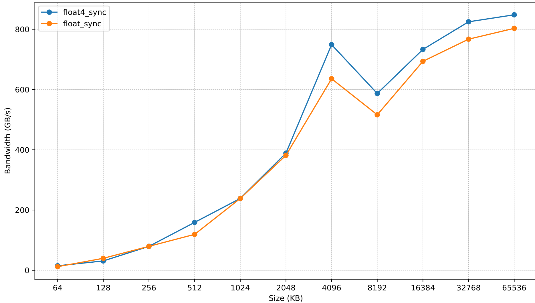
Bandwidth: Global->Shared
