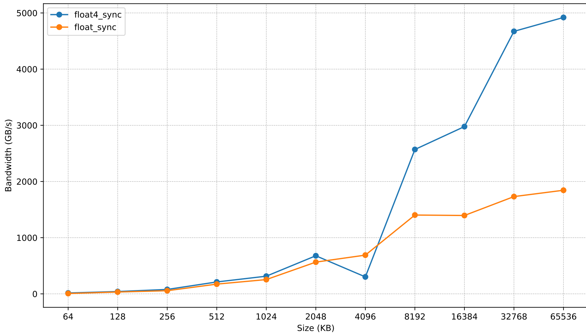
Bandwidth: Global->Shared
