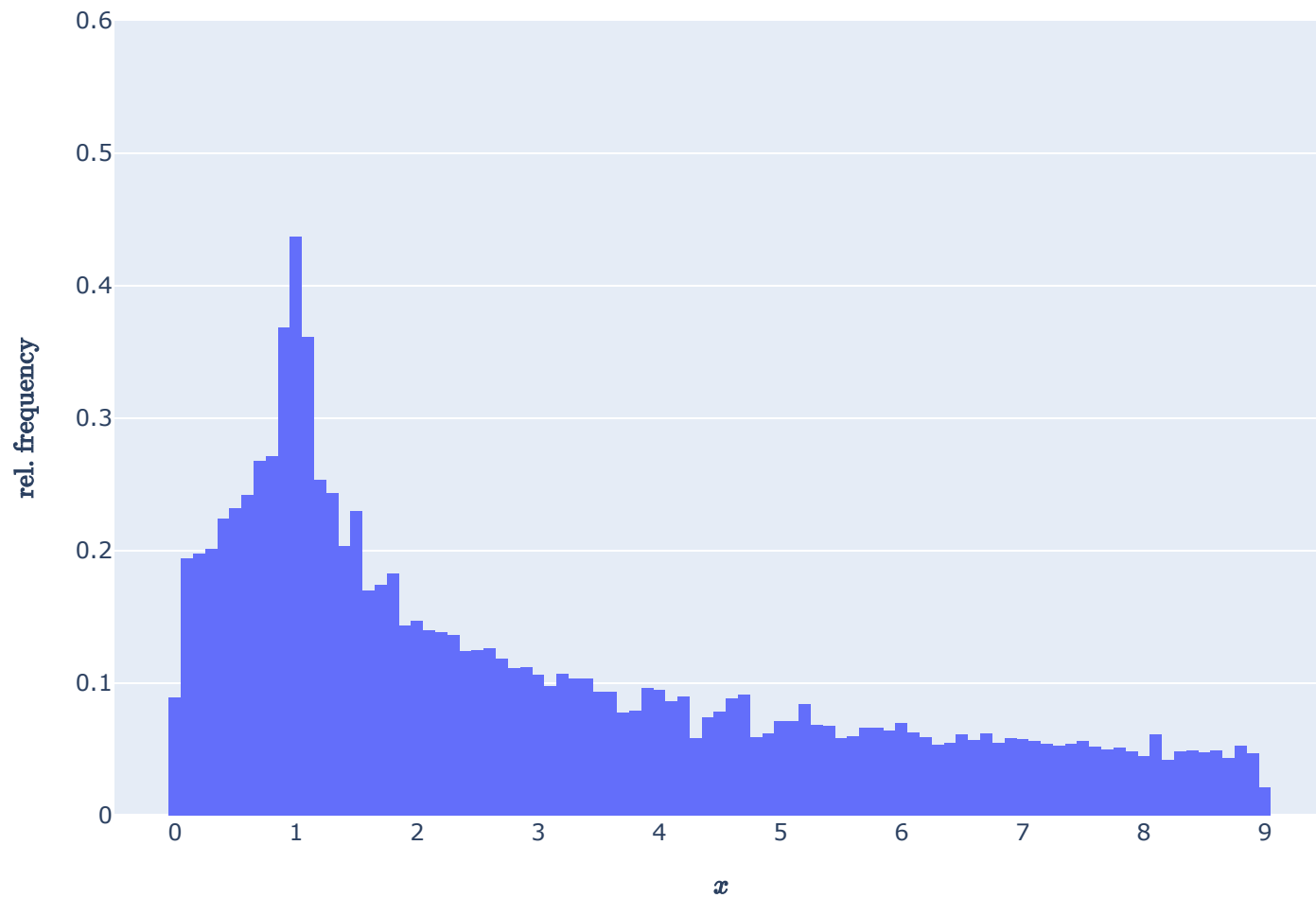
Normalized Histogram of dual GF_{24000}
