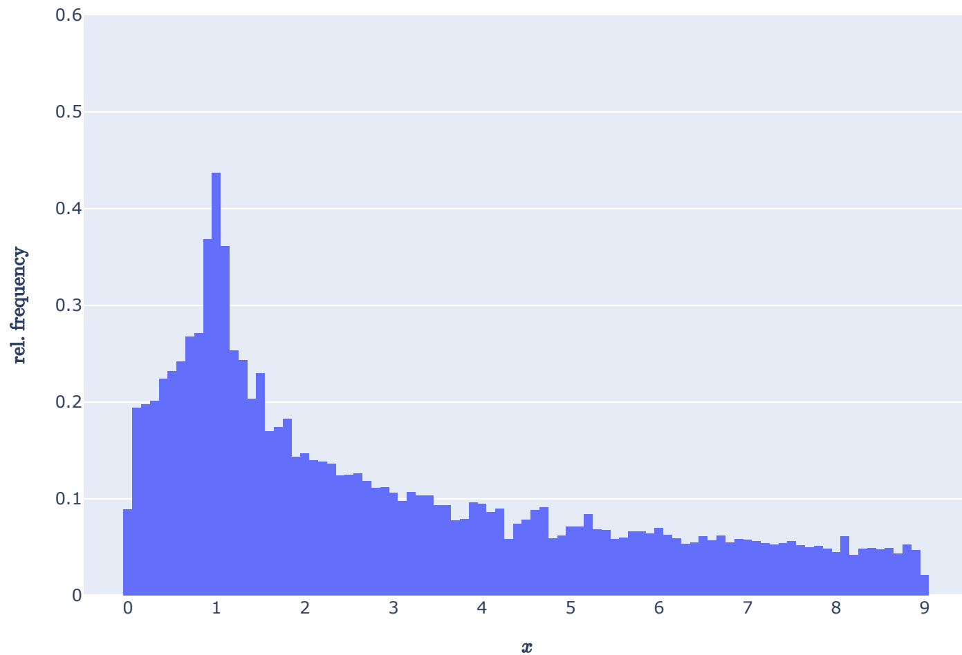
Normalized Histogram of dual GP_{24000}
