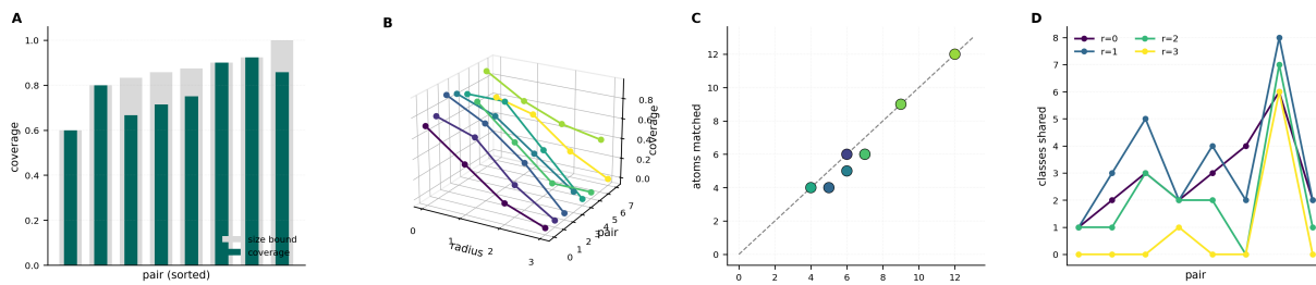
Figure 3: Correspondence on one-position matched pairs, and the same radius erosion seen in the correspondence itself rather than in the overlap. Correspondence is computed without search (Theorem 3.4); it is not a maximum common substructure and carries no connectivity guarantee (Section 6). (A) Coverage (teal) against the size bound \min(n_1, n_2) / \max(n_1, n_2) (grey) per pair, sorted. Mean coverage is 0.776 with median 0.775 and minimum 0.600, and 3 of the 8 pairs sit exactly at their ceiling — every atom of the smaller structure found a correspondent. Raw coverage therefore understates match quality for pairs of unequal size, and normalising by the bound is a correction we have not applied. (B) Coverage against radius for each matched pair in three dimensions. Mean coverage falls 0.776 \rightarrow 0.599 \rightarrow 0.295 \rightarrow 0.076 across radii 0–3: the same monotone erosion Figure 1 shows for overlap, now visible in the number of atoms actually paired. By radius 3 the matcher pairs almost nothing. (C) Atoms matched against the atom count of the smaller structure, with the identity line and colour by coverage. Points on the line are the three pairs at their size bound; the vertical drop for the others is the number of atoms the substitution displaced far enough in cut-key terms to break the correspondence. (D) Classes shared between the two structures of each pair at each radius. The curves fall together rather than crossing, so no pair is anomalously robust to refinement — the erosion is a property of the labelling, not of particular molecules.
