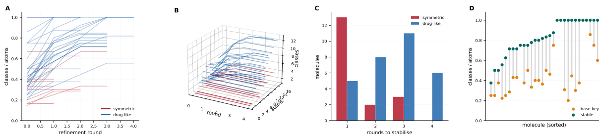
Figure 1: Refinement is monotone, saturates within four rounds, and stops at a level set by the molecule rather than by the number of rounds available. Each round applies (2) and the resulting partition is an invariant at every round by Theorem 4.4; the curves below are therefore not a convergence toward an answer but a sequence of successively finer correct answers. (A) Classes divided by atoms against round, one line per molecule, symmetric corpus red and drug-like blue. Every trajectory is non-decreasing — Theorem 4.2 — and flat after its stabilisation round. The two corpora separate cleanly: the symmetric set saturates at mean 0.477 (minimum 0.167) and the drug-like set at mean 0.823 (minimum 0.375). The gap is not a difference in how hard the two sets are; it is the symmetry the red molecules possess and the blue ones largely do not. (B) The same trajectories against heavy-atom count in three dimensions. The drug-like surface rises with size while the symmetric surface stays low irrespective of it: benzene at six atoms and anthracene at fourteen both stabilise at a handful of classes. Class count is therefore not a function of molecular size, which is what distinguishes Theorem 4.5 from a mere resolution limit. (C) Rounds to stabilisation. The symmetric corpus is concentrated at one round (13 of 18) and the drug-like corpus spreads over one to four; the median across both is 2 and the maximum is 4, well inside the |I| bound of Theorem 4.2. Symmetric molecules stabilise sooner because there is less for refinement to find. (D) Per molecule, base-key ratio (orange) and stable ratio (teal) joined by a segment, sorted by the stable value. The mean rises from 0.505 to 0.823, a mean lift of 0.318 and a maximum of 0.800, and 12 of 30 molecules reach 1.0. Both endpoints matter to the argument: the orange points show the base key is not a ranking, and the 18 teal points short of 1.0 show the stable partition is not one either.
