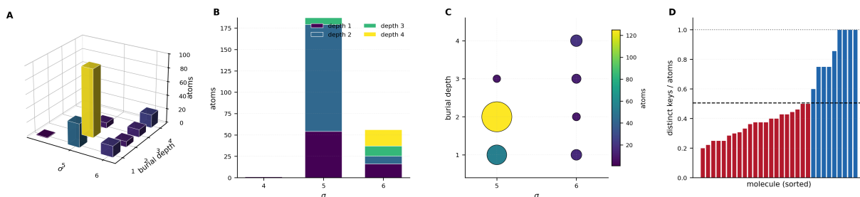
Figure 3: The base cut key is a genuine invariant and a very coarse one: it occupies eight cells of a small discrete space and separates barely half the atoms of a typical structure. All quantities are computed on contact graphs (Theorem 2.1) with strictly positive weights; every separation cost is an exact minimum cut obtained by maximum flow (Theorem 2.2), so the small number of distinct values below is a property of the invariant and not of a tolerance or a rounding rule. (A) Occupancy of the (\sigma, d, \text{heavy degree}) cells over the 244 heavy atoms of the drug-like corpus, bar height and colour both the atom count. Thirteen cells are occupied; the largest holds 98 atoms and the smallest holds 1. The realised ranges are \sigma \in \{4, 5, 6\} , d \in \{1, 2, 3, 4\} and degree \in \{1, 2, 3\} , so the key takes far fewer values than the 36 the ranges alone would permit — the components are strongly dependent, which is why the figure is an occupancy plot rather than a scatter. (B) The same atoms decomposed by burial depth within each \sigma level. At \sigma = 5 the depths run 53/125/8 over depths 1–3 and at \sigma = 6 they run 16/9/12/19 over depths 1–4. Depth therefore separates atoms that \sigma alone does not, which is the whole reason Theorem 2.2 takes a pair rather than a scalar; a key built from \sigma alone would realise three values across the entire corpus. (C) The (\sigma, d) plane with marker area and colour proportional to occupancy: eight distinct base keys, populated between 1 and 125 atoms. The extreme unevenness is the quantitative form of Theorem 3.2 operating far beyond genuine symmetry — most of these coincidences are not orbits, they are the invariant’s coarseness, and Section 4 exists to address them. (D) Distinct base keys divided by heavy atoms, one bar per molecule sorted ascending; dashed line the corpus mean 0.505, dotted line the value 1.0 a canonical ranking requires. The ratio runs 0.200–1.000 with median 0.414; 21 of 30 molecules fall below the mean and only 4 reach 1.0. This is the measurement that makes the paper’s subject non-trivial: had these bars sat near the dotted line, the base key would already be a ranking and Section 4 would be unnecessary.
