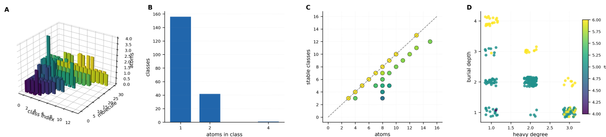
Figure 4: Class structure of the stable partition: mostly singletons, with the multi-atom classes concentrated at genuinely symmetric positions. All panels are over the drug-like corpus at the stable partition P^* (Theorem 4.3); 199 classes over 244 atoms. (A) Atoms per class index for every molecule, one row of bars per molecule ordered by size. The surface is dominated by unit-height bars; the taller bars are the positions refinement declines to split, and they occur in the molecules carrying ring or substituent symmetry rather than uniformly across the corpus. (B) Distribution of class sizes: 156 singletons, 42 classes of two, and a single class of four. That the tail is this short is the reason the stable ratio reaches 0.823 rather than saturating lower — most drug-like atoms are in fact structurally distinct, and the invariant says so. (C) Stable classes against heavy-atom count, coloured by their ratio, with the identity diagonal. Points on the diagonal are molecules refinement fully separates; the vertical gap for points below it is the number of atoms their symmetry protects. (D) Burial depth against heavy degree for all 244 atoms, jittered for visibility and coloured by \sigma . The \sigma levels occupy visibly different regions of the (degree, depth) plane, so the two components of Theorem 2.2 are not redundant: depth carries information about an atom’s embedding that neither \sigma nor degree supplies alone, and it is the component with no counterpart in a conventional element-and-degree atom identifier.
