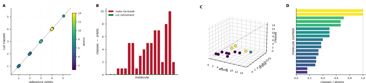
Figure 2: On every molecule of the symmetric corpus the stable partition is exactly the automorphism orbit partition — neither coarser nor finer. Reference orbit counts are determined by inspection of the constitutional graph and were fixed before comparison; they are stated per molecule in the corpus source with the reasoning for each. Two were initially wrong and were corrected against the measurement (Section 5), which is weaker evidence than a correct prediction against a correct reference and is marked as such. (A) Cut classes against reference orbits, coloured by heavy-atom count, jittered slightly so coincident points stay visible. All eighteen lie on the identity diagonal. The corpus spans 1–5 orbits and 1–14 heavy atoms, so the agreement is not an artefact of a narrow range. (B) Residual classes minus orbits per molecule for the cut refinement (green) against the index tie-breaking control (red). The green residual is identically zero; the red exceeds the orbit count by up to 10 classes on the same molecules, mean excess 3.72. Plotting the two together is what makes the flat green line informative rather than merely empty. (C) Atoms, orbits and classes in three dimensions with the identity line drawn and points coloured by rounds to stabilisation. The points lie in the plane classes = orbits and well below the atom-count diagonal, which is Theorem 4.5 and its converse holding simultaneously on this corpus: the partition is bounded above by the orbit count and here attains it. (D) Classes divided by atoms per molecule, sorted, running 0.167–1.000. Values far below the dotted line at 1.0 are molecules whose own symmetry the refinement declines to break; benzene at 1/6 is the extreme. A canonical ordering would place every bar at 1.0, which is precisely the behaviour Theorem 4.5 forbids.
