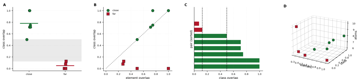
Figure 2: Separation of the annotated groups at the working radius. (A) Class overlap for the two groups with horizontal bars at the group means; the shaded band is the gap between the highest far value (0.125) and the lowest close value (0.500), which no pair occupies. (B) Class overlap against element overlap per pair with the identity line: the two far points on the floor at element overlap 0.5 and 1.0 are pairs an element-keyed comparison cannot distinguish and the cut class separates completely. (C) All ten pairs sorted by class overlap, with the two dashed lines marking the boundaries of the empty band. (D) Element overlap, class overlap and structure size in three dimensions, showing that the separation is not an artefact of the pairs having different sizes.
