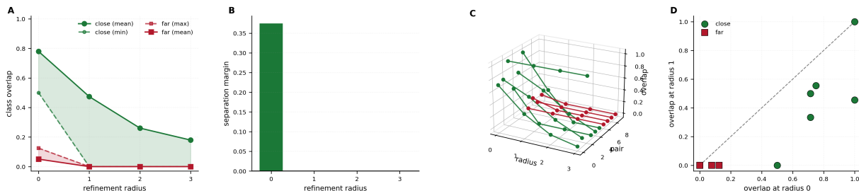
Figure 1: Tolerance is a resolution parameter: the coarsest radius separates best. (A) Mean class overlap against refinement radius for the close (green) and far (red) groups, with the shaded bands running to the minimum close and maximum far value; the bands are disjoint only at radius 0. (B) The separation margin, minimum close minus maximum far, by radius: +0.375 at radius 0 and exactly 0 at radii 1, 2 and 3. (C) Every annotated pair traced across all four radii in three dimensions, close in green and far in red; the close traces descend toward the far floor as radius grows. (D) Overlap at radius 1 against overlap at radius 0 for each pair, with the identity line; every close pair falls below the diagonal, and one falls to zero.
