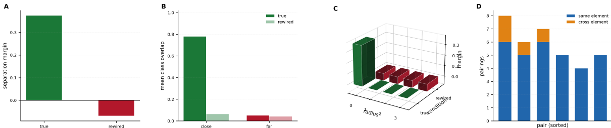
Figure 4: The rewiring control and the cross-element gain. (A) Separation margin for the true structures (+0.375) and after rewiring the second structure of each pair at random while holding atom composition and edge count fixed (−0.069): the separation does not survive. (B) Group means before and after rewiring; the close mean collapses from 0.780 to near the far value, while the far mean barely moves. (C) Margin over radius under both conditions in three dimensions: the true margin exists only at radius 0 and the rewired margin is negative everywhere. (D) Pairings admitted per close pair split into same-element (blue) and cross-element (orange); the cross-element pairings, which an element-keyed matcher cannot make, total 4 across the six pairs and occur in three of them.
