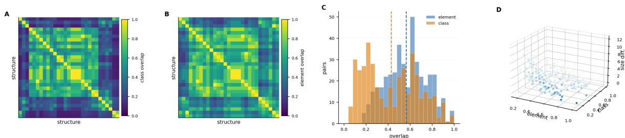
Figure 5: Class and element overlap over the drug-like set. (A) Class-overlap matrix for all \binom{30}{2} pairs of the drug-like corpus at radius 0, structures in corpus order. (B) Element-overlap matrix for the same pairs on the same scale; the block structure differs visibly, so the two quantities are not proxies for one another. (C) Distributions of the two overlaps over the 406 pairs with their means marked: class overlap is shifted toward lower values, because agreeing on composition is easier than agreeing on structural role. (D) Element overlap, class overlap and absolute size difference in three dimensions, coloured by class minus element overlap; points far from the diagonal plane are pairs on which the two criteria most disagree.
