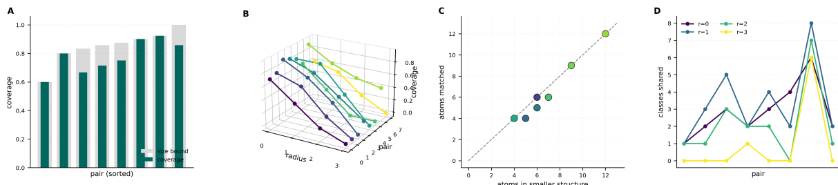
Figure 3: Correspondence on matched pairs and its decay with radius. (A) Coverage (teal) against the size bound \min(n_1, n_2) / \max(n_1, n_2) (grey) per pair, sorted; three of the eight pairs reach their ceiling, so raw coverage understates the match quality for pairs of unequal size. (B) Coverage against radius for each matched pair in three dimensions; every pair loses coverage monotonically as the labelling discriminates more. (C) Atoms matched against the atom count of the smaller structure, with the identity line and colour by coverage; points on the line are pairs in which every atom of the smaller structure found a correspondent. (D) Classes shared between the two structures of each pair at each radius, showing the same erosion from a different quantity.
