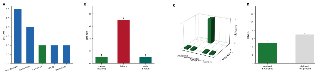
Figure 4: Eight probes realise five distinct verdict labels, and no failure verdict carries a value. (A) Labels realised by the probe set. empty appears here only because of defect D4: the parser raised on empty input before clause (V2) was reached, so empty was unreachable from the SMILES path and an empty record was reported as malformed . That is the conflation Theorem 5.6 identifies, occurring inside the implementation built to prevent it; Theorem 9.3 gives the account. (B) Probes by whether their label may carry a value, whether the label is a failure, and whether a value was in fact carried. One probe is value-bearing, seven are failures, and exactly one carried a value — the same one. The failure column is the population in which a violation could occur, and it is empty. (C) Each probe positioned by label, by whether its label may carry a value, and by whether it did. Every bar sits at did carry = 0 except the single translated probe, and no bar sits in the region ( may carry = 0, did carry = 1) that would constitute a violation. That region is empty by construction as well as by measurement: the invariant is enforced in the verdict constructor, so this panel confirms the constructor is reached rather than establishing the property independently. (D) Labels realised by these probes against those defined but not probed. Five of twelve are exercised. The unexercised seven are plan-level and honjo-level labels outside the translation path, and we make no claim about them here.
