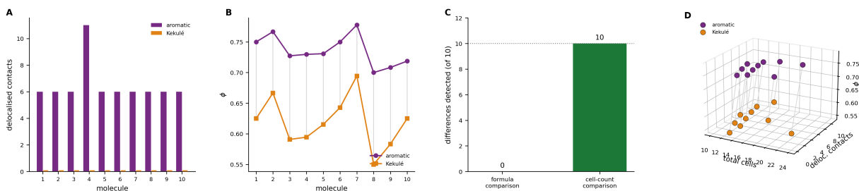
Figure 3: Ten molecules written two faithful ways yield ten pairs of contact graphs that differ, while formula-level comparison reports agreement on all ten. Each molecule is expressed once with a lower-case aromatic ring and once in an alternating Kekulé assignment. Both translations state exactly what their source states, so neither is a misreading. (A) Delocalised contacts under each reading. The aromatic form yields six per benzenoid ring (eleven for naphthalene); the Kekulé form yields none, drawn as explicit floor ticks so the zeros read as measured rather than missing. By Theorem 3.8 neither graph converts into the other without supplying a fact. (B) The supplied fraction under each reading, joined per molecule. The Kekulé form is lower in every case — benzene gives 0.750 against 0.625 — because stating per-contact cell counts removes them from what convention must supply. The gap is a measurement of how much the aromatic notation leaves to the reader. (C) What each comparison detects. A formula-level comparison finds 0 of 10 differences; a cell-count comparison finds 10 of 10. This is the paper’s central practical claim in one measurement: the disagreement is real and the conventional instrument is blind to it, which is why Section 9.7 argues identity comparison is the wrong tool here. (D) The two readings in (total cells, delocalised contacts, \phi ) space, joined per molecule. The two clouds are disjoint on every axis, and the connecting segments are all parallel: the disagreement is systematic, not sporadic. Note that the measured ratio is 10/10 because these pairs were constructed to contain an aromatic ring; Theorem 9.4 states that this measures visibility and not prevalence.
