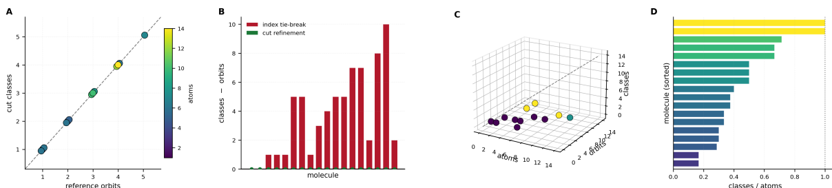
Figure 3: On every molecule of the symmetric corpus the stable partition is exactly the automorphism orbit partition — neither coarser nor finer. Reference orbit counts are determined by inspection of the constitutional graph and were fixed before comparison; they are stated per molecule in the corpus source with the reasoning for each. Two were initially wrong and were corrected against the measurement (Section 5), which is weaker evidence than a correct prediction against a correct reference and is marked as such. (A) Cut classes against reference orbits, coloured by heavy-atom count, jittered slightly so coincident points stay visible. All eighteen lie on the identity diagonal. The corpus spans 1–5 orbits and 1–14 heavy atoms, so the agreement is not an artefact of a narrow range. (B) Residual classes minus orbits per molecule for the cut refinement (green) against the index tie-breaking control (red). The green residual is identically zero; the red exceeds the orbit count by up to 10 classes on the same molecules, mean excess 3.72. Plotting the two together is what makes the flat green line informative rather than merely empty. (C) Atoms, orbits and classes in three dimensions with the identity line drawn and points coloured by rounds to stabilisation. The points lie in the plane classes = orbits and well below the atom-count diagonal, which is Theorem 4.5 and its converse holding simultaneously on this corpus: the partition is bounded above by the orbit count and here attains it. (D) Classes divided by atoms per molecule, sorted, running 0.167–1.000. Values far below the dotted line at 1.0 are molecules whose own symmetry the refinement declines to break; benzene at 1/6 is the extreme. A canonical ordering would place every bar at 1.0, which is precisely the behaviour Theorem 4.5 forbids.
