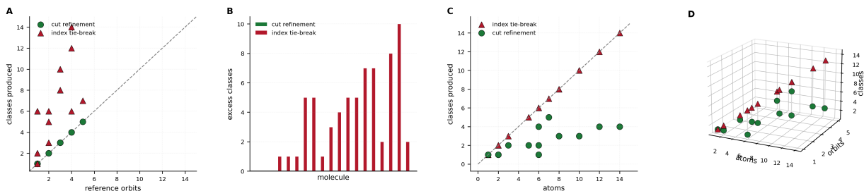
Figure 4: The negative control: a procedure identical to ours except that it breaks ties by atom index destroys the orbit structure on 16 of 18 molecules. The control differs from the construction in exactly one respect — it appends the atom’s index to its cut key — which is what a canonical ordering does. If it did not fail, Figure 3 would be testing nothing. (A) Classes produced against reference orbits for the cut refinement (green circles) and the control (red triangles). The green points lie on the diagonal; the red rise above it and continue rising with molecular size rather than with symmetry. (B) Excess classes over the reference for both procedures per molecule. The control over-separates on 16 of 18 molecules, by up to 10 classes; the two it does not are the single-heavy-atom cases, where there is nothing to separate. The refinement over-separates on none, which is Theorem 4.5 as a measurement rather than as a proof. (C) Classes produced against heavy-atom count. The control tracks the atom-count diagonal exactly, because an ordering must assign a distinct rank to every atom; the refinement does not, and the vertical distance between the two point sets is the symmetry the ordering has discarded. (D) Both procedures in the (atoms, orbits, classes) space, joined per molecule by a vertical segment. Segment length is the control’s over-separation and grows with molecular size while the green endpoints stay pinned to the orbit plane. The figure is the paper’s central distinction rendered geometrically: an invariant lives in a plane fixed by the molecule, an ordering on a diagonal fixed by the atom count.
