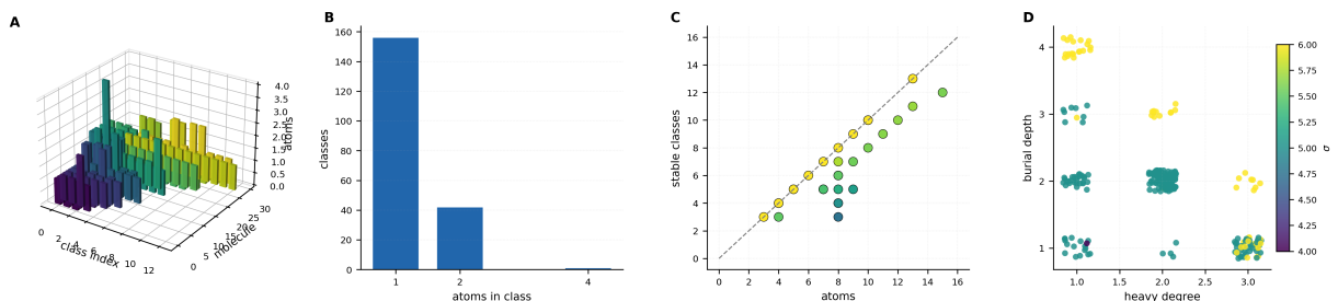
Figure 5: Class structure of the stable partition: mostly singletons, with the multi-atom classes concentrated at genuinely symmetric positions. All panels are over the drug-like corpus at the stable partition P^* (Theorem 4.3); 199 classes over 244 atoms. (A) Atoms per class index for every molecule, one row of bars per molecule ordered by size. The surface is dominated by unit-height bars; the taller bars are the positions refinement declines to split, and they occur in the molecules carrying ring or substituent symmetry rather than uniformly across the corpus. (B) Distribution of class sizes: 156 singletons, 42 classes of two, and a single class of four. That the tail is this short is the reason the stable ratio reaches 0.823 rather than saturating lower — most drug-like atoms are in fact structurally distinct, and the invariant says so. (C) Stable classes against heavy-atom count, coloured by their ratio, with the identity diagonal. Points on the diagonal are molecules refinement fully separates; the vertical gap for points below it is the number of atoms their symmetry protects. (D) Burial depth against heavy degree for all 244 atoms, jittered for visibility and coloured by \sigma . The \sigma levels occupy visibly different regions of the (degree, depth) plane, so the two components of Theorem 2.2 are not redundant: depth carries information about an atom’s embedding that neither \sigma nor degree supplies alone, and it is the component with no counterpart in a conventional element-and-degree atom identifier.
