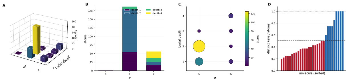
Figure 1: The base cut key is a genuine invariant and a very coarse one: it occupies eight cells of a small discrete space and separates barely half the atoms of a typical structure. All quantities are computed on contact graphs (Theorem 2.1) with strictly positive weights; every separation cost is an exact minimum cut obtained by maximum flow (Theorem 2.2), so the small number of distinct values below is a property of the invariant and not of a tolerance or a rounding rule. (A) Occupancy of the (\sigma, d, \text{heavy degree}) cells over the 244 heavy atoms of the drug-like corpus, bar height and colour both the atom count. Thirteen cells are occupied; the largest holds 98 atoms and the smallest holds 1. The realised ranges are \sigma \in \{4, 5, 6\} , d \in \{1, 2, 3, 4\} and degree \in \{1, 2, 3\} , so the key takes far fewer values than the 36 the ranges alone would permit — the components are strongly dependent, which is why the figure is an occupancy plot rather than a scatter. (B) The same atoms decomposed by burial depth within each \sigma level. At \sigma = 5 the depths run 53/125/8 over depths 1–3 and at \sigma = 6 they run 16/9/12/19 over depths 1–4. Depth therefore separates atoms that \sigma alone does not, which is the whole reason Theorem 2.2 takes a pair rather than a scalar; a key built from \sigma alone would realise three values across the entire corpus. (C) The (\sigma, d) plane with marker area and colour proportional to occupancy: eight distinct base keys, populated between 1 and 125 atoms. The extreme unevenness is the quantitative form of Theorem 3.2 operating far beyond genuine symmetry — most of these coincidences are not orbits, they are the invariant’s coarseness, and Section 4 exists to address them. (D) Distinct base keys divided by heavy atoms, one bar per molecule sorted ascending; dashed line the corpus mean 0.505, dotted line the value 1.0 a canonical ranking requires. The ratio runs 0.200–1.000 with median 0.414; 21 of 30 molecules fall below the mean and only 4 reach 1.0. This is the measurement that makes the paper’s subject non-trivial: had these bars sat near the dotted line, the base key would already be a ranking and Section 4 would be unnecessary.
