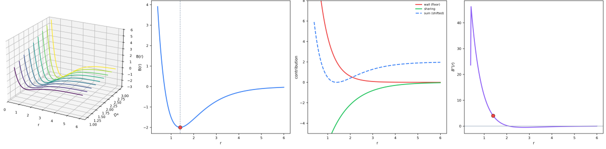
Figure 5: Bond Length as the Convex Thickness Minimiser. (A) Three-dimensional family of joint-thickness wells B(r) = D_e[(1 - e^{-d(r-r_0)})^2 - 1] over internuclear separation r and well depth D_e (viridis), each curve a convex well with a single interior minimum; the minimum deepens with D_e but never moves to r = 0 . (B) The thickness profile B(r) (blue) with its unique interior minimiser marked (red point at r^* = 1.40 , in units of r_0 ); the dashed line locates r^* . The curve diverges as r \rightarrow 0 and plateaus as r \rightarrow \infty , the equilibrium standoff of Theorem 5.1. (C) The two competing contributions: the repulsive wall (red, diverging as r \rightarrow 0 —the contact floor asserting itself), the sharing pull (green, the boundary-reduction drawing the atoms together), and their sum (blue dashed) with the interior minimum, showing the floor as the origin of short-range repulsion. (D) Curvature B''(r) (purple) versus separation; it is positive at the minimiser (red point) and crosses zero only well away from it, confirming the well is locally convex at r^* ( B''(r^*) = 3.99 > 0 ).
