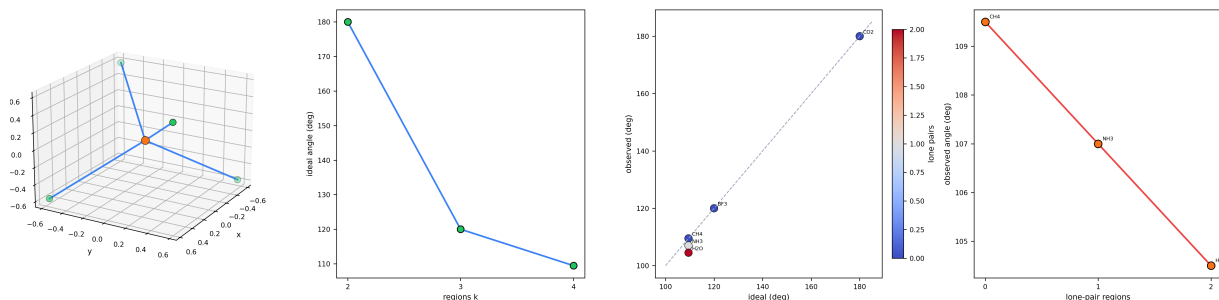
Figure 7: Molecular Geometry as Maximal Angular Separation. (A) Three-dimensional rendering of the four maximally separated bond directions of a four-coordinate centre (methane): bonds (blue) from the central atom (orange) to the four ligand directions (green) at the regular-tetrahedron vertices, the configuration that minimises pairwise solid-angle overlap (Theorem 6.4). (B) Ideal symmetric bond angle versus number of interface regions k : 180^\circ ( k = 2 , linear), 120^\circ ( k = 3 , trigonal planar), 109.47^\circ ( k = 4 , tetrahedral)—the maximal-separation angles of k points on the sphere. (C) Observed versus ideal symmetric angle for five molecules, coloured by lone-pair count (coolwarm); points on the diagonal (grey dashed) are the lone-pair-free backbones ( \text{CO}_2 , \text{BF}_3 , \text{CH}_4 ), and points below it are the lone-pair-compressed geometries ( \text{NH}_3 , \text{H}_2\text{O} ). (D) Observed angle of the four-region family versus lone-pair count: 109.5^\circ ( \text{CH}_4 , none) \rightarrow 107^\circ ( \text{NH}_3 , one) \rightarrow 104.5^\circ ( \text{H}_2\text{O} , two), the monotone compression as unshared regions are added.
