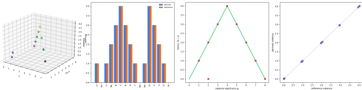
Figure 3: Valence as the Vacancy Count. (A) Three-dimensional scatter of the sixteen elements in (\nu, C_v - \nu, \text{valence}) space—vacancy against co-vacancy against derived valence—coloured by valence (viridis). The points lie on the surface \text{valence} = \min(\nu, C_v - \nu) , the covalent-valence rule of Theorem 4.1. (B) Derived valence (blue) and reference common valence (orange) as grouped bars per element. The two series coincide for every element, the 16/16 agreement of the validation suite. (C) The closure curve \min(\nu, 8 - \nu) (green) over valence-electron count q_v , with the elements (red points) sitting on it; the curve peaks at four, recovering carbon’s valence of four at q_v = 4 . (D) Derived versus reference valence on the identity diagonal (grey dashed); all points lie on the diagonal (small jitter added for visibility), confirming exact reproduction of the common valences from the vacancy arithmetic alone.
