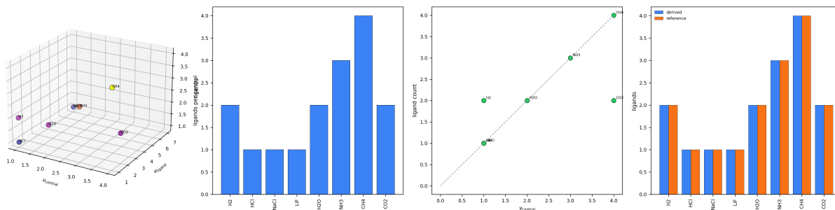
Figure 4: Stoichiometry from Vacancy Matching. (A) Three-dimensional scatter of eight molecules in (\nu_{\text{central}}, \nu_{\text{ligand}}, \text{ligand count}) space, points labelled by molecule and coloured by ligand count (plasma). The ligand count is fixed by closing the central atom’s vacancy through interfaces of the ligand’s vacancy, recovering the observed formulae. (B) Ligands per central atom for H 2 , HCl, NaCl, LiF, H 2 O, NH 3 , CH 4 , CO 2 , showing the 1:1, 2:1, 3:1, 4:1 ratios as the central vacancy increases. (C) Central vacancy \nu_{\text{central}} versus predicted ligand count; the points track the diagonal (grey dashed) for the hydride series (H 2 O, NH 3 , CH 4 ), where each monovalent ligand closes one central vacancy. (D) Derived (blue) versus reference (orange) ligand count per molecule as grouped bars; the two coincide for all eight molecules (8/8), the vacancy ratio reproducing each stoichiometry with no further input.
