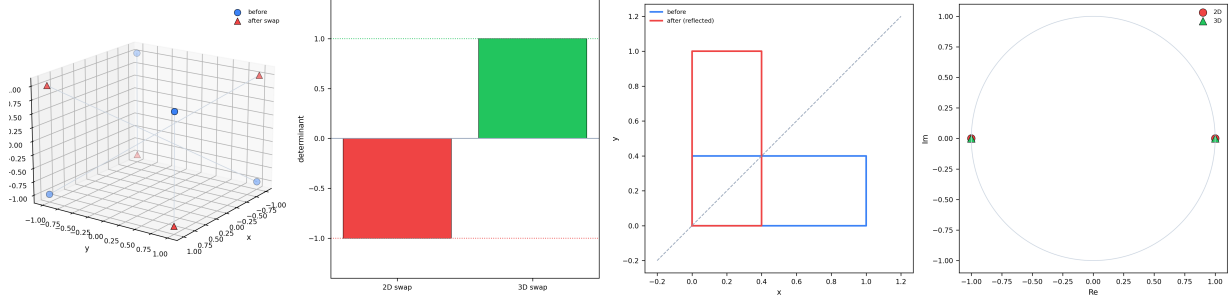
Figure 6: Three Dimensions and the Absence of a Privileged Axis. (A) Three-dimensional action of the axis-swap (x, y, z) \mapsto (y, x, -z) on the vertices of a tetrahedron: original vertices (blue) and their images (red triangles) joined by displacement lines. The swap is realised as a continuous proper rotation, exchanging the two axes by an internal motion (Principle 6.1). (B) Determinants of the axis-swap matrices: the two-dimensional swap has determinant -1 (a reflection, red) and the three-dimensional swap has determinant +1 (a proper rotation in SO(3) , green), the dashed guides marking \pm 1 . (C) The two-dimensional swap as a reflection across the line y = x (grey dashed): a rectangle (blue) mapped to its mirror image (red), showing that in d = 2 exchanging the axes requires a reflection, not an internal rotation—hence an external choice. (D) Eigenvalue spectra of the two swap matrices on the unit circle (grey): the two-dimensional swap (red) has eigenvalues \pm 1 , the three-dimensional swap (green triangles) has eigenvalues consistent with a proper rotation, confirming d = 3 as the minimum dimension of selector-free axis exchange.
