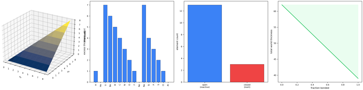
Figure 8: Why a World of Bounded Atoms Must Be a World of Molecules. (A) Three-dimensional surface of the shareable content \min(\nu_a, \nu_b) over the vacancy plane (cividis): the boundary that two atoms can commit jointly, zero whenever either is closed-shell and rising with the smaller vacancy, the resource from which structure is built. (B) Excess boundary thickness \kappa\phi(\nu) above the closed-shell minimum for sixteen elements, bars red where \nu = 0 (no excess: the noble-gas minimum) and blue where \nu > 0 (excess to be relaxed by bonding). (C) Element census of the open (reactive, blue) versus closed (inert, red) shells among the sixteen elements, the count of atoms that carry shareable vacancy versus those that do not. (D) Total world boundary thickness versus the fraction of open atoms that have bonded: the monotone decrease (green, shaded reduction) shows that a world of bounded atoms with positive vacancy lowers its total thickness by forming molecules—chemical structure as the floor’s economy (Theorem 8.1).
