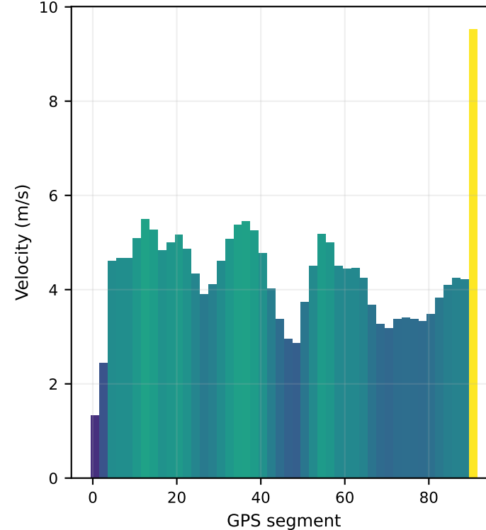
(c) Runner velocity profile
