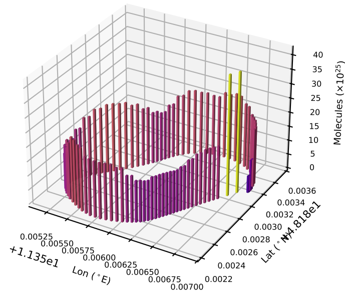
(b) Molecular displacement
