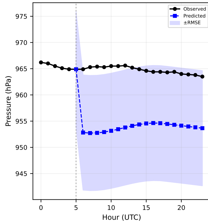
(c) Pressure (RMSE=10.98 hPa)
