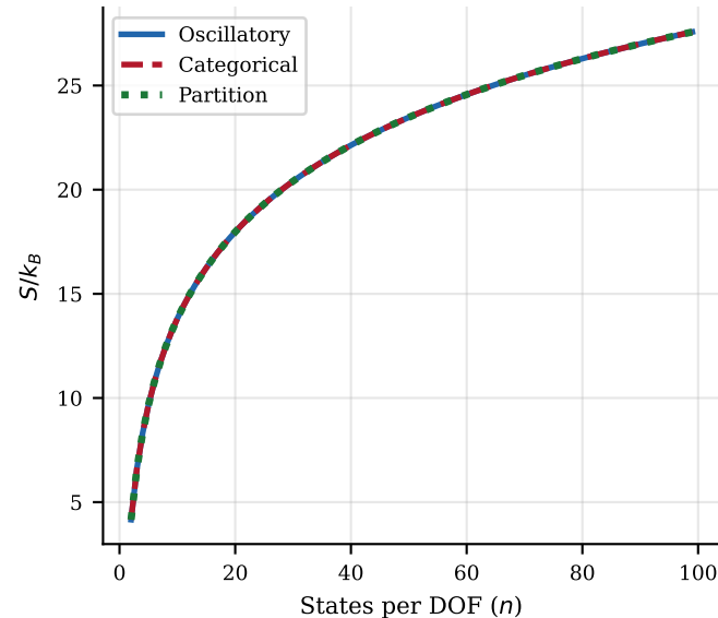
(B) Triple Equivalence ( M = 6 )
