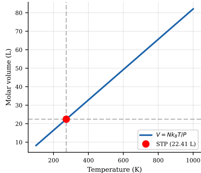
(C) Ideal gas from Triple Equiv.
