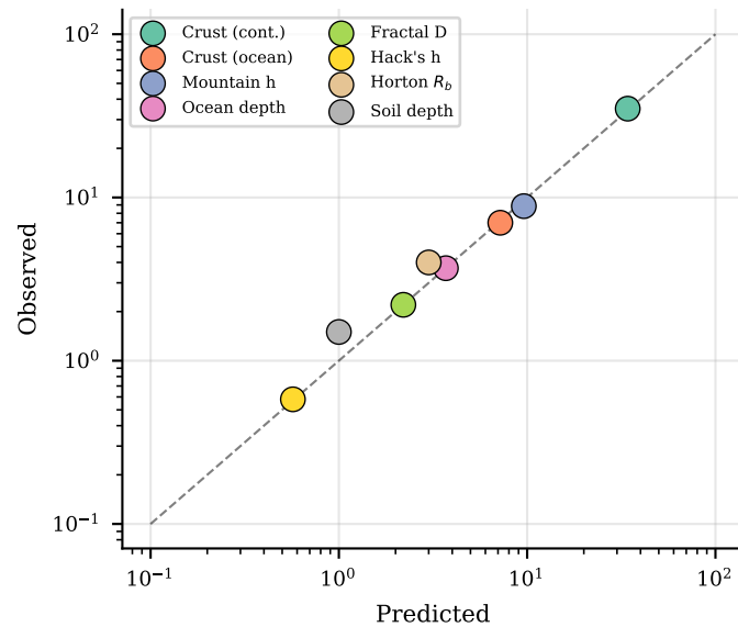
(B) Derived vs Observed
