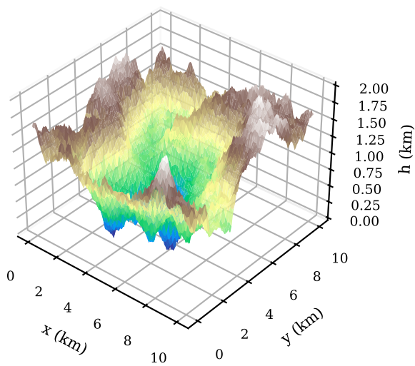
(A) Synthetic terrain ( D = 2.25 )
