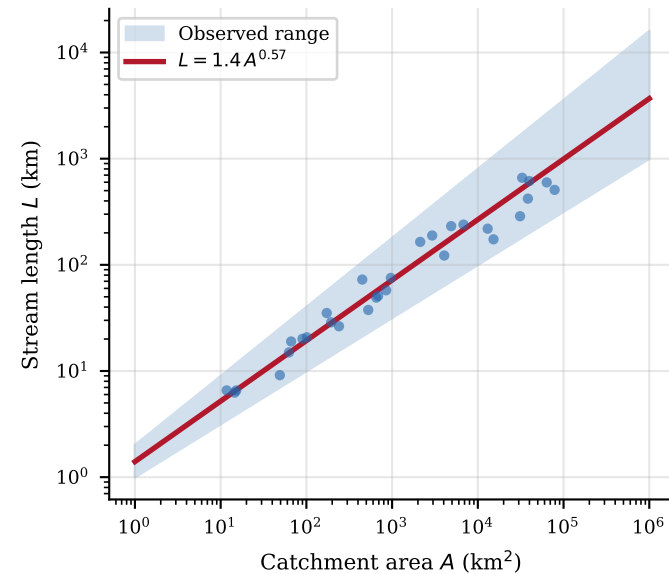
(C) Hack's law
