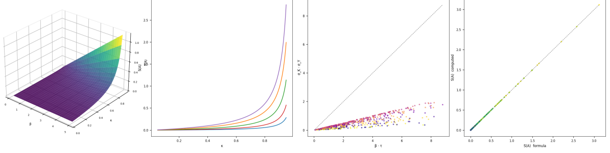
Figure 5: Agent Triple and Receiver Uncertainty: Agent Floor Surface, Floor-Contraction Family, Uncertainty Product, and Formula Verification. (A) Three-dimensional surface of the agent floor \bar{S}(\mathcal{A}) = \beta \cdot \sigma \kappa / ((1 - \kappa) \Sigma) over receiver floor \beta \in [0.1, 5.0] and contraction ratio \kappa \in [0.05, 0.92] , with fixed \sigma = 2 and \Sigma = 100 . The surface is bilinear in the flat (\beta, \kappa) directions when \kappa is small, but curves sharply upward as \kappa \rightarrow 1 : the divergence of \kappa/(1 - \kappa) amplifies even small receiver floors into large agent floors for high-contraction methodologies. (B) Agent floor \bar{S}(\mathcal{A}) versus contraction ratio \kappa for five receiver floors \beta \in \{0.5, 1.0, 2.0, 3.5, 5.0\} , with \sigma = 3.0 and \Sigma = 100 . Each curve is monotone increasing and convex in \kappa , diverging as \kappa \rightarrow 1 . The vertical gap between adjacent curves is \Delta \bar{S} = \Delta \beta \cdot \sigma \kappa / ((1 - \kappa) \Sigma) , growing with \kappa : heterogeneity in receiver floors is amplified by the methodology’s contraction ratio. (C) Receiver Uncertainty Principle: scatter of \sigma_K \cdot \sigma_Y = (\alpha \beta) \cdot ((1 - \alpha) \tau) against the bound \beta \tau for N = 600 triples (\beta, \tau, \alpha) with \alpha drawn uniformly from [0.05, 0.95] . The colour encodes \alpha . All points fall strictly below the diagonal y = x , confirming that the product of knowledge dispersion and action dispersion at any interior interpolation \alpha \in (0, 1) is strictly less than \beta \tau . (D) Formula verification: computed agent floor \bar{S}(\mathcal{A}) = \beta \cdot (\sigma \kappa / (1 - \kappa)) / \Sigma versus the same quantity computed by separating the receiver and methodology components, for N = 300 random (\beta, \kappa, \sigma) triples.
