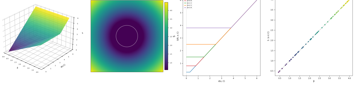
Figure 1: S-Functional Geometry: Floor Surface, Spatial Field, Family of Floors, and Cell-Truth Attainment. (A) Three-dimensional surface of the S-functional S(\beta, d) = \max(\beta, d(x, C)) over a grid of receiver floors \beta \in [0.1, 4.0] and distances d(x, C) \in [0, 6] . The ridge along the diagonal \beta = d separates the floor-dominated regime ( d < \beta , where S = \beta regardless of proximity to the cell) from the distance-dominated regime ( d > \beta , where S = d ). (B) Spatial heatmap of S(\mathcal{R}, x; C) for a ball cell C = B(\mathbf{0}, r) with r = 1.2 and floor \beta = 0.6 in \mathbb{R}^2 . The white circle marks the cell boundary \partial C . Inside C the field is constant at \beta (the Cell-Truth property: x \in C \Rightarrow S = \beta ), while outside it grows monotonically with \|x\| , saturating to \|x\| - r + \beta for large \|x\| . (C) S-functional versus distance d(x, C) for five floors \beta \in \{0.3, 0.8, 1.5, 2.5, 3.8\} . Each curve is piecewise linear with a kink at d = \beta : when d < \beta the curve is horizontal at height \beta so the floor dominates, and when d > \beta the curve rises with unit slope so distance dominates. (D) Cell-Truth attainment: S-functional values at N = 60 randomly drawn in-cell states for 60 receivers with floors \beta \in [0.2, 4.0] , plotted against \beta . Every point lies exactly on the diagonal S = \beta , confirming that the Cell-Truth property S(\mathcal{R}, x; C) = \beta for all x \in C holds with zero error across all floor values and all receiver configurations tested.
