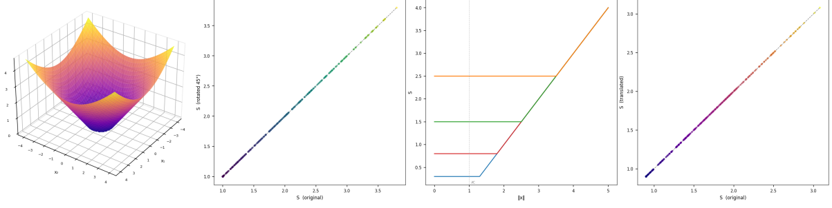
Figure 2: Representational Invariance: Distance Field, Rotation Isometry, Floor Family at the Cell Boundary, and Translation Isometry. (A) Three-dimensional surface of the cell-distance function d(x_1, x_2; C) = \max(0, \|x\| - r) for C = B(\mathbf{0}, 1) in \mathbb{R}^2 . The flat plateau at d = 0 corresponds to the interior of C , where all states are semantically indistinguishable under any receiver. The surrounding cone rises with unit slope in the Euclidean norm. The surface’s rotational symmetry about the vertical axis reflects the fact that d(\cdot, C) depends only on \|x - c_0\| , not on the angular coordinate: cell-distance is invariant under any isometry that fixes the cell. (B) Representational Invariance (rotation): scatter of S(\mathcal{R}, x; C) against S(\mathcal{R}, \phi(x); \phi(C)) for N = 400 query points and a 45-degree rotation \phi . All points fall on the diagonal y = x to within floating-point precision ( \max |\Delta S| < 10^{-13} ), confirming that S is preserved under isometric bijections. (C) S -functional versus \|x\| (Euclidean norm of x ) for four floors \beta \in \{0.3, 0.8, 1.5, 2.5\} . The vertical dotted line at \|x\| = r = 1 marks the cell boundary. Inside the cell ( \|x\| < r ), S = \beta is constant. Outside ( \|x\| > r ), S increases linearly with slope 1. (D) Representational Invariance (translation): scatter of S(\mathcal{R}, x; C) against S(\mathcal{R}, x + c; C + c) for N = 400 query points and shift c = (2.3, -1.7) .
