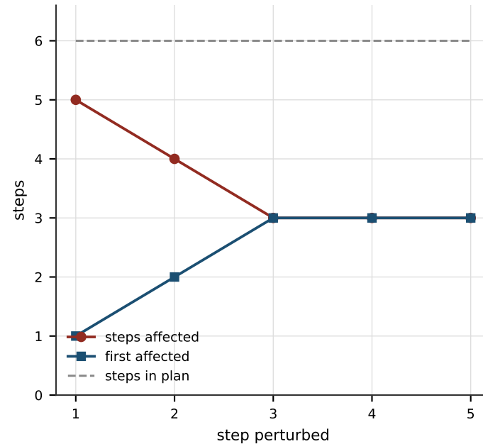
(c) perturbation is confined downstream
