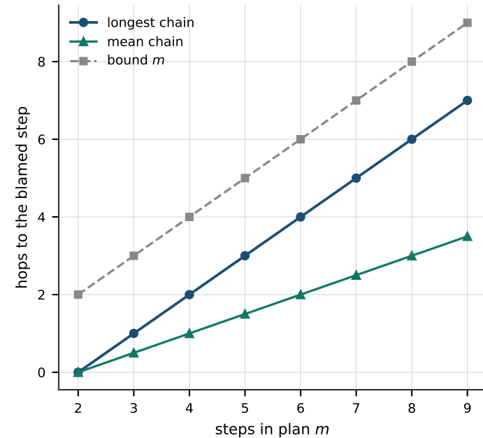
(a) blame terminates within m
