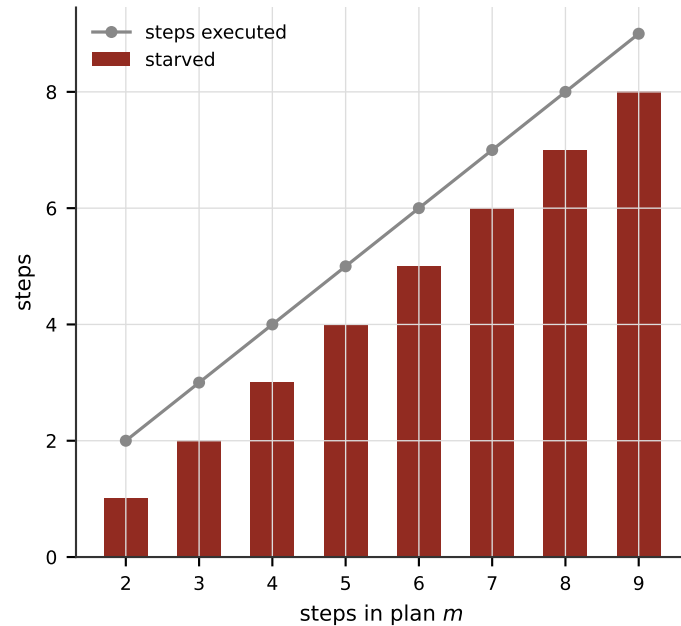
(b) starvation spreads downstream
