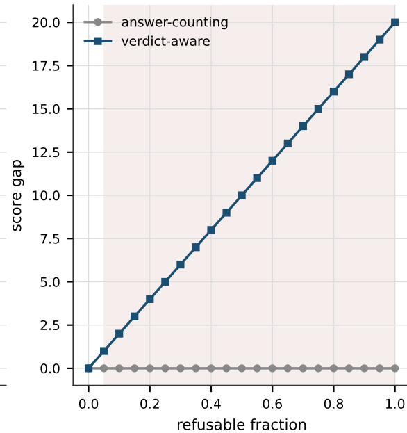
(c) separation; shaded = rankings disagree
