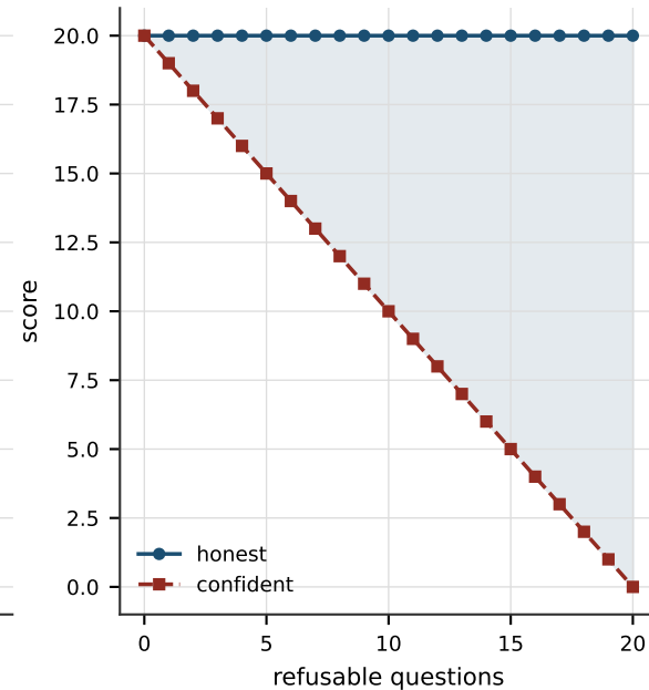
(b) verdict-aware rule
