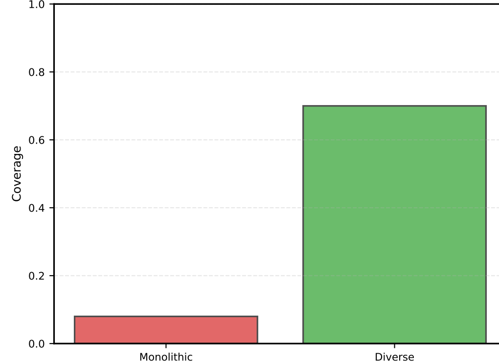
C. Coverage
