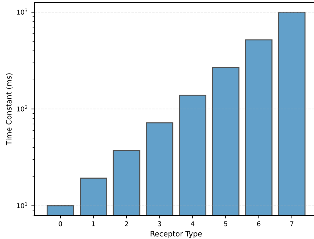
A. Distribution
