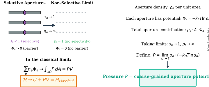
(D) Classical Limit: Non-Selective Apertures (E) Pressure: Emergent from Aperture Statistics
