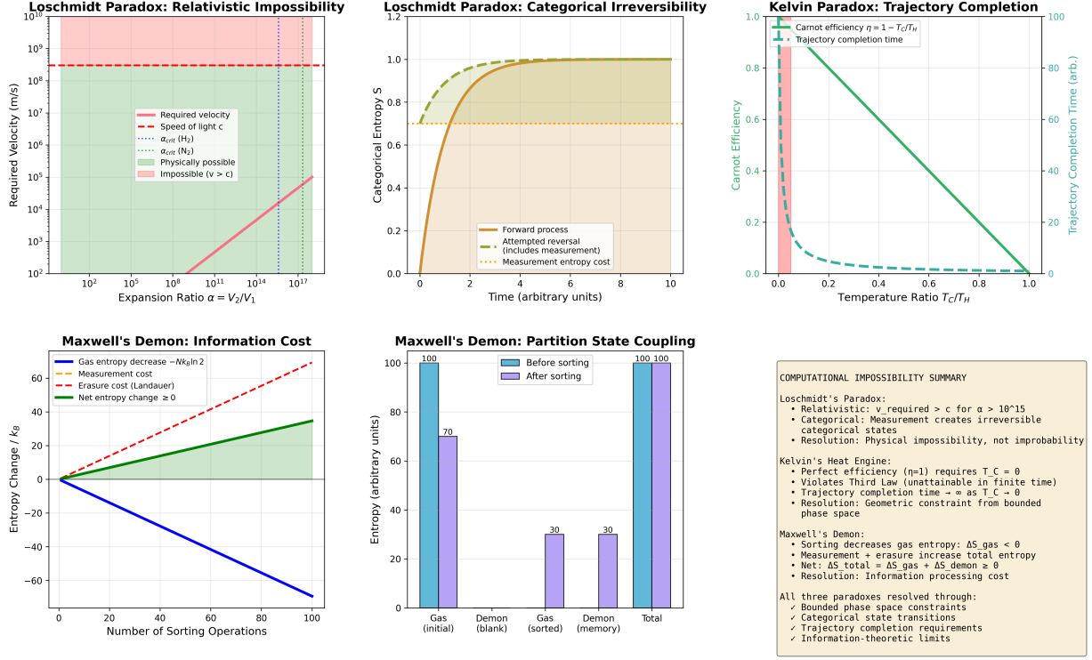
Figure 11: Resolution of three classical paradoxes through categorical constraints. (Top left) Loschmidt paradox—relativistic impossibility: required velocity (pink curve) for phase space reversal exceeds speed of light c (red dashed) at expansion ratio a = V_2/V_1 > 10^{14} . Critical velocities for H_2 (purple dotted) and N_2 (green dotted) mark molecular-specific thresholds. Green shaded region: physically possible; red shaded region: impossible ( v > c ). (Top center) Loschmidt paradox—categorical irreversibility: categorical entropy S (orange curve) increases monotonically during forward process, saturating at S \approx 1.0 . Attempted reversal (green dashed) including measurement creates additional entropy (orange shaded region). Measurement entropy cost (yellow dotted) prevents return to S = 0 . (Top right) Kelvin paradox—trajectory completion: Carnot efficiency \eta = 1 - T_C/T_H (green curve) approaches unity as T_C \rightarrow 0 , but trajectory completion time (cyan dashed) diverges to \infty (right axis). Red shaded region: thermodynamically forbidden. (Bottom left) Maxwell's demon—information cost: gas entropy decrease -Nk_B \ln 2 (blue curve) is offset by measurement cost (red dashed) and erasure cost (orange, Landauer). Net entropy change \geq 0 (green curve, shaded). (Bottom center) Maxwell's demon—partition state coupling: before sorting, gas entropy is 100 units (cyan bar), demon memory is blank (purple bar, 0 units). After sorting, gas entropy decreases to 70 units, but demon memory increases to 30 units. Total entropy remains 100 units. (Bottom right) Summary box: All three paradoxes resolved through bounded phase space constraints, categorical state transitions, trajectory completion requirements, and information-theoretic limits.
