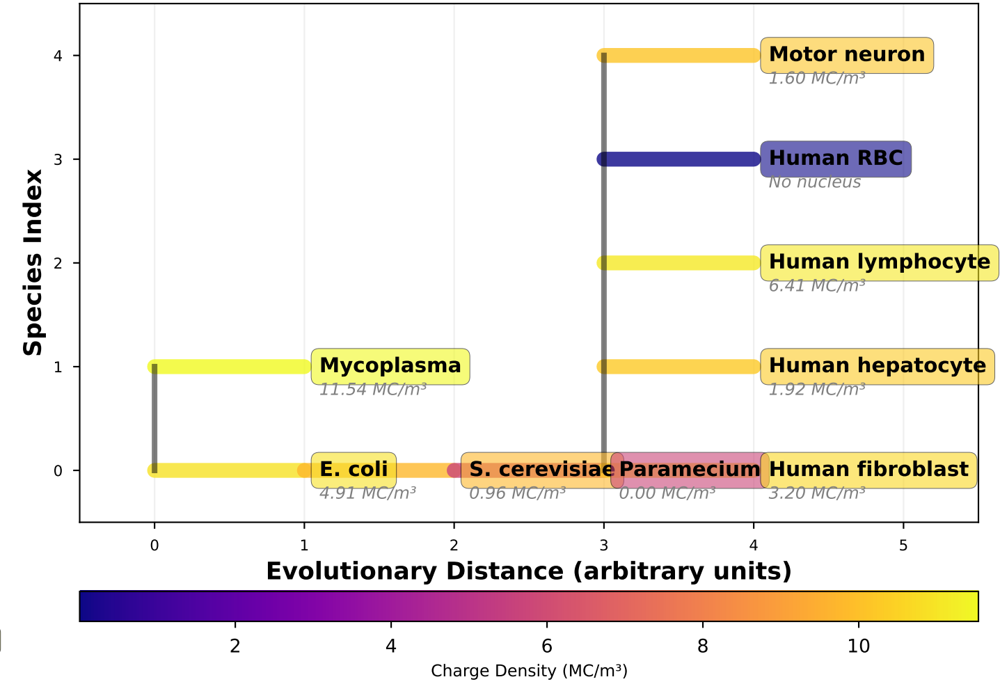
(B) Phylogenetic Tree: Charge Density Conservation
