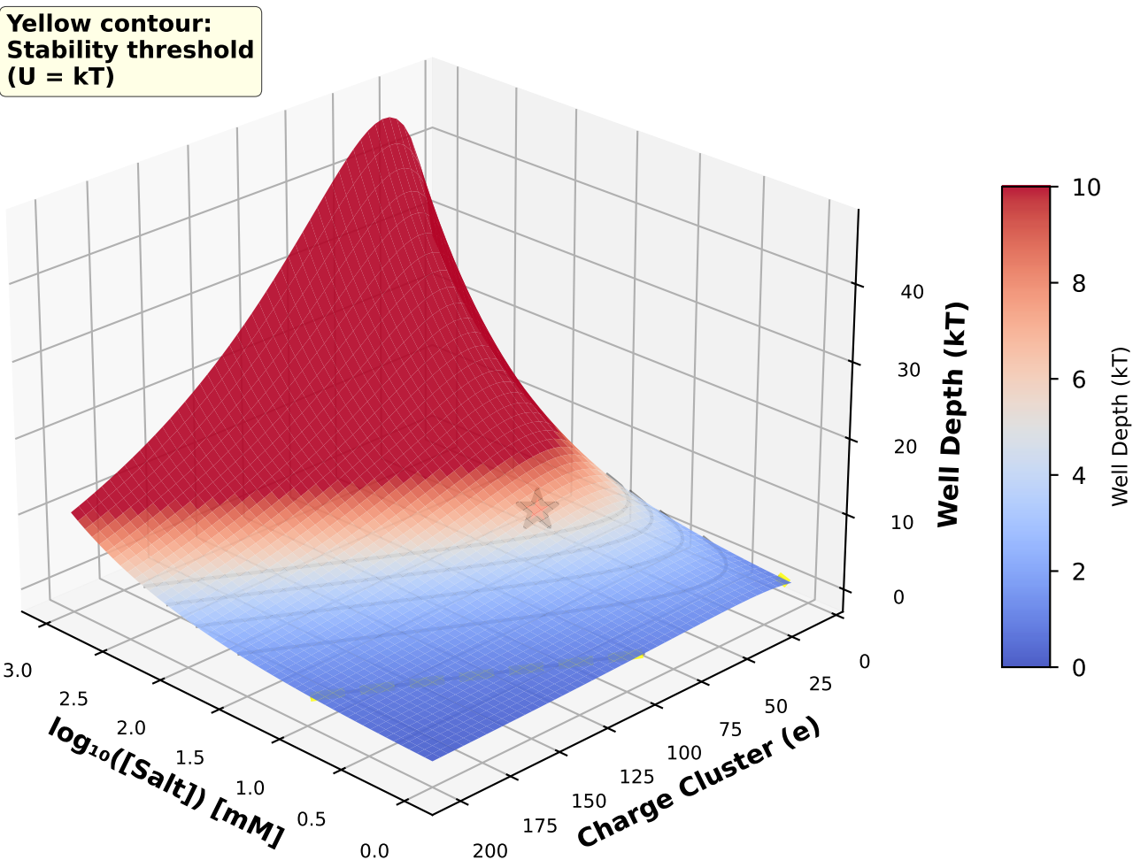
(C) Chamber Stability Landscape
