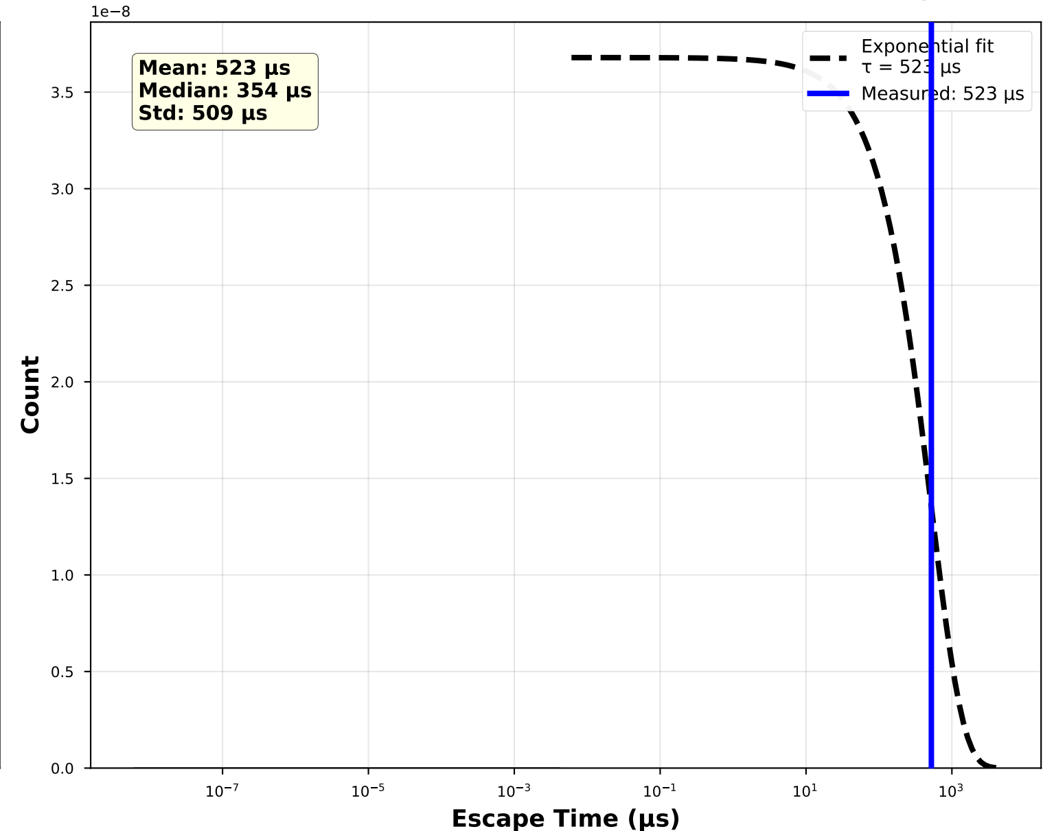
(B) Chamber Lifetime Distribution: Kramers Theory
