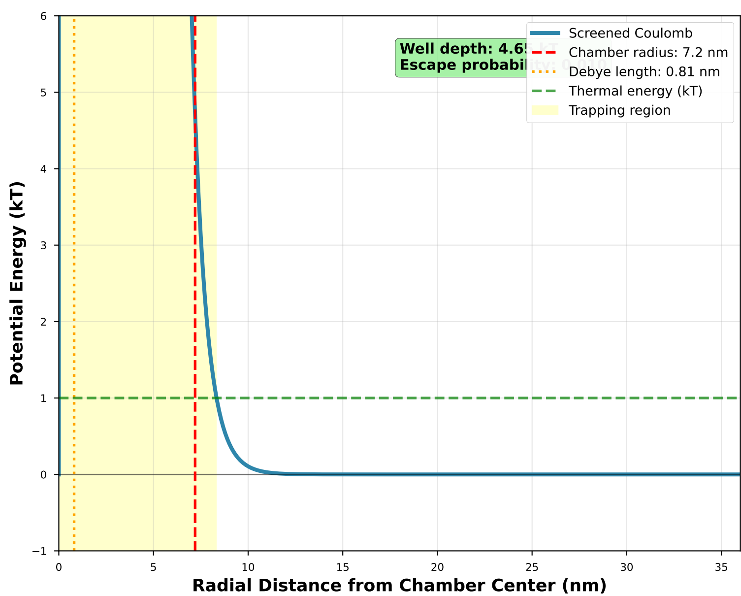
(A) Electrostatic Potential Well: 4.7 kT Depth
